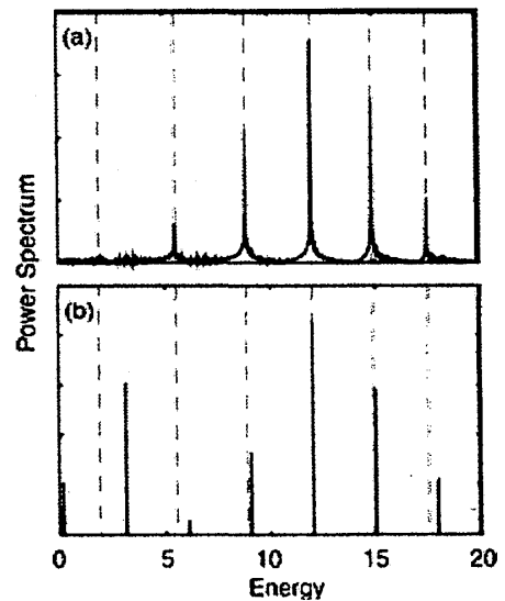
Fig.1 Semiclassical spectra
