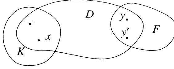
FIGURE 5. The global boundary Harnack principle in terms of the Green function.
