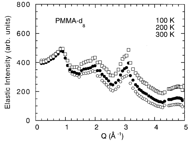
FIG. 4. Q dependence of the coherent elastic scattering from PMMA- d_8 at 100 ( \square ), 200 ( \bullet ), and 300 ( \circ ) K. Three distinct peaks at 0.9, 2.0, and 3.1 \text{ \AA}^{-1} were observed in the Q range. According to the assignment by Lovell and Windle (Ref. 30), the peak at 0.9 \text{ \AA}^{-1} is a composition containing neighboring interchain correlation and intrachain correlation between nearest-neighboring ester groups in a syndiotactic sequence of atactic PMMA, and the second and third peaks at 2.0 and 3.1 \text{ \AA}^{-1} are intrachain correlations between neighboring ester and methyl groups in a syndiotactic sequence and between nearest-neighboring methylene units in a chain, respectively.
