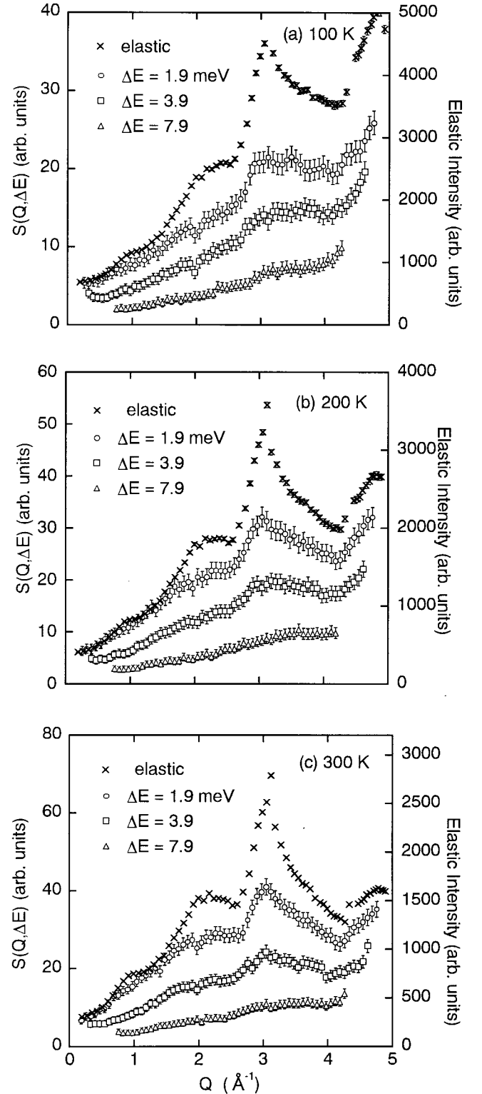
FIG. 5. Q dependence of the coherent inelastic scattering from PMMA- d_8 as a function of the energy transfer \Delta E from 1.9 to 7.9 meV. (a) 100 K, (b) 200 K, and (c) 300 K. The spectra were obtained by integrating S(Q, \Delta E) in an energy range from \Delta E - 0.5 to \Delta E + 0.5 meV. The Q dependence of the coherent elastic scattering I_{\text{el}}(Q) is also plotted in a form of Q^2 I_{\text{el}}(Q) .
