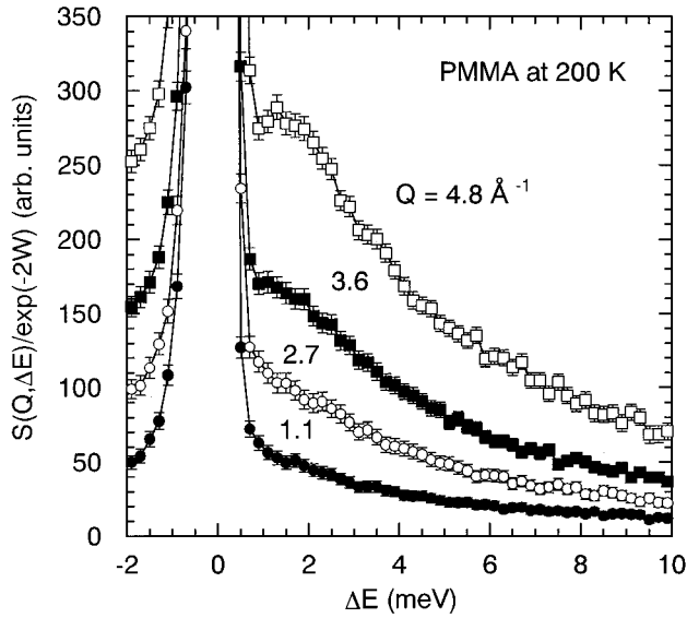
FIG. 2. Incoherent dynamic scattering laws S(Q, \Delta E) of PMMA at 200 K ( T_g = 377 K) as a function of Q from 1.1 to 4.8 \text{ \AA}^{-1} . S(Q, \Delta E) was corrected for the Debye-Waller factor \exp(-2W) . Note that the onset temperature of the fast process is approximately 160 K.
