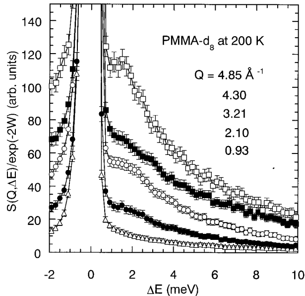
FIG. 3. Coherent dynamic scattering laws S(Q, \Delta E) of PMMA- d_8 at 200 K as a function of Q from 0.93 to 4.85 \text{ \AA}^{-1} . S(Q, \Delta E) was corrected for the Debye-Waller factor \exp(-2W) .
