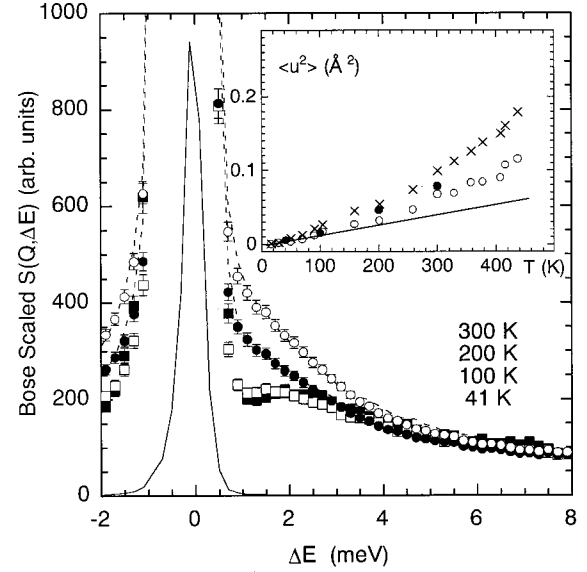
FIG. 1. Incoherent dynamic scattering laws S(Q, \Delta E) of PMMA at Q = 2.48 \text{ \AA}^{-1} scaled to a reference temperature ( =100 \text{ K} ) by the Bose factor after correcting for the Debye-Waller factor evaluated from the Q dependence of the incoherent inelastic scattering intensity. The inset shows the temperature dependence of the mean-square displacement \langle u^2 \rangle evaluated from the Q dependence of the incoherent elastic scattering with various energy resolution \delta E . ( \times ) \delta E = 0.08 \text{ meV} (Ref. 28), ( \circ ) \delta E = 2 \text{ meV} (Ref. 28), and ( \bullet ) \delta E = 0.16 \text{ meV} (this work).
