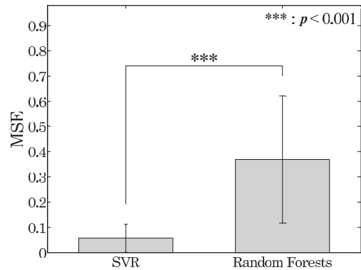
Fig. 4 Comparison of average MSE
