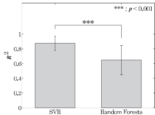
Fig. 5 Comparison of average R^2
