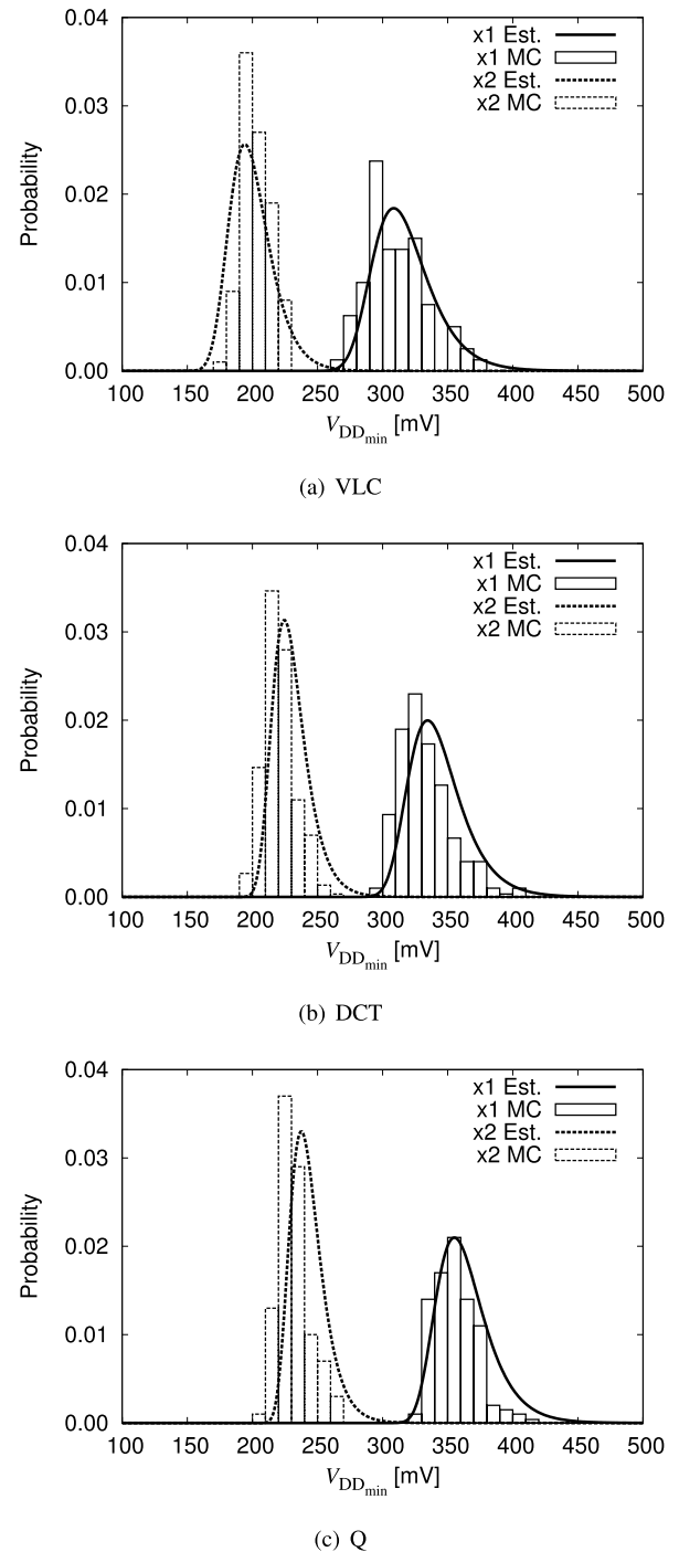
Fig. 10 Estimated V_{\text{DDmin}} distributions using the proposed model (Step 1 of the proposed design strategy), and the histograms obtained by SPICE Monte Carlo simulations. The result for W: \times 1.5 is omitted for visibility because it largely overlaps to the results of the other two sized transistors.
