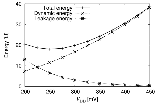
Fig. 2 One-period energy of a 101-stage inverter-chain ring oscillator as a function of supply voltage ( V_{DD} ).
