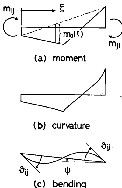
Fig. 2 Distribution diagrams of a girder.
