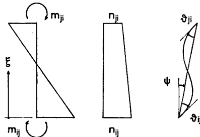
(a) moment (b) axial force (c) bending
