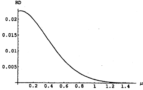
(e) n_1 = n_2 = 10, \sigma_1^2 = 1, \sigma_2^2 = 1 .
