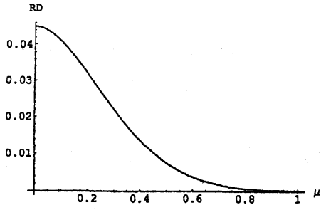
(a) n_1 = n_2 = 11, \sigma_1^2 = 1, \sigma_2^2 = 0.1^2 .
