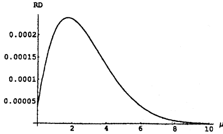
(c) n_1 = n_2 = 11, \sigma_1^2 = 1, \sigma_2^2 = 10^2 .
