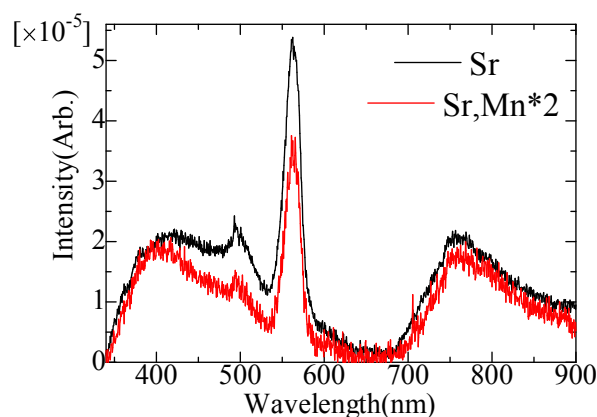
Fig. 2 Photoluminescence spectra of synthesized calcite with an impurity of Sr and Sr + Mn.
