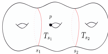
FIGURE 7. Two commuting separating Dehn twists
