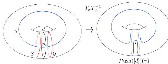
FIGURE 2. The point-pushing map \mathcal{P}\text{ush}
