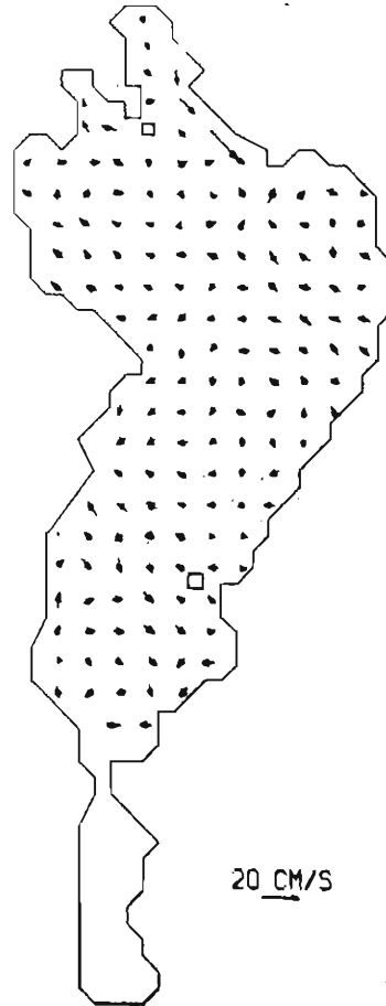
Fig. 18. Horizontal velocities at 6000 minutes after falling down of wind.
