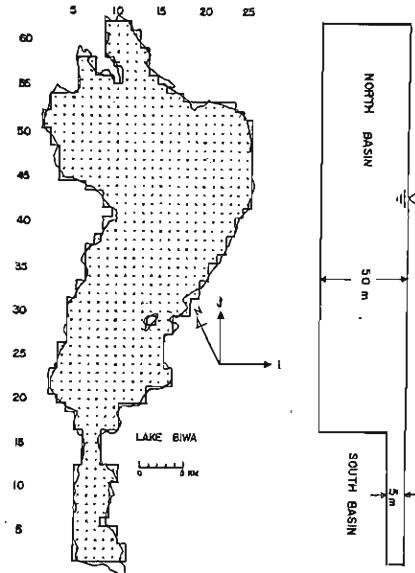
Fig. 2. Computational grid and longitudinal cross-section of model Lake Biwa.
