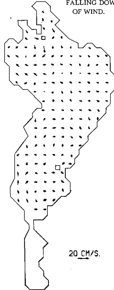
Fig. 17. Horizontal velocities at 4800 minutes after falling down of wind.
