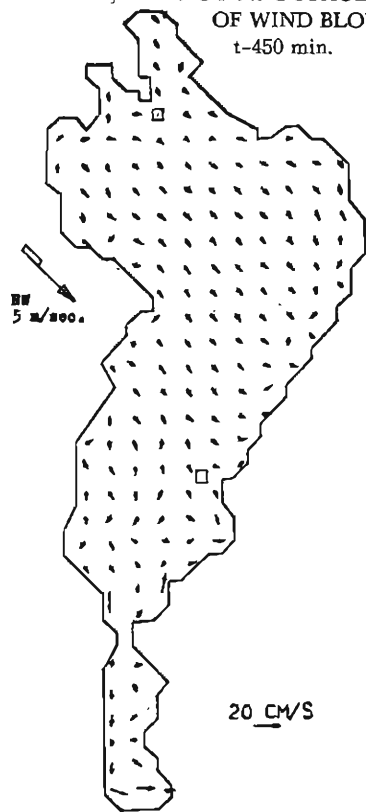
Fig. 16. Horizontal velocities at the final stage of wind blow.
