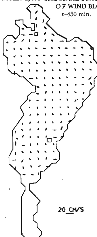
Fig. 16. Horizontal velocities at the final stage of wind blow.
