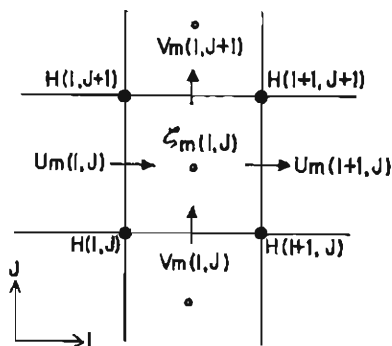
Fig. 4. Computational grid employed in model Lake Biwa. Black circles denote depth points; open circles indicate elevation points. Arrows indicate flow points.
