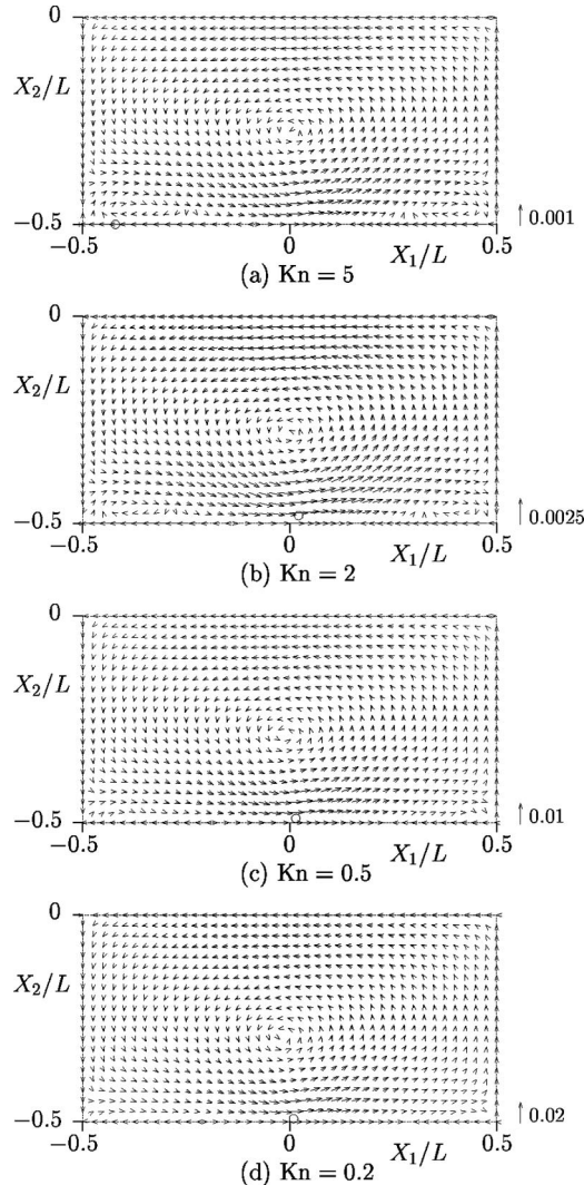
FIG. 3. Flow induced in the lower half of the container for T_2/T_1 = 2 . (a) Kn = 5 , (b) Kn = 2 , (c) Kn = 0.5 , (d) Kn = 0.2 . The arrow indicates the two-dimensional flow velocity vector (v_1, v_2)/(2RT_1)^{1/2} at its starting point. The reference length of the arrow is shown in the right margin of each figure. The symbol \circ indicates the point with the maximum flow speed.
