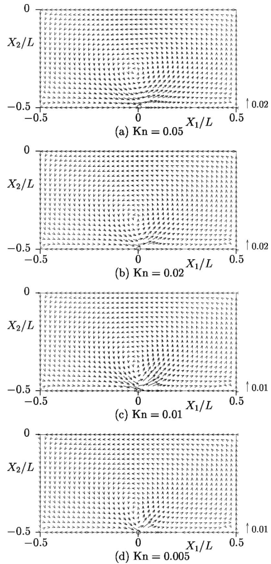
FIG. 4. Flow induced in the lower half of the container for T_2/T_1 = 2 . (a) Kn = 0.05 , (b) Kn = 0.02 , (c) Kn = 0.01 , (d) Kn = 0.005 . See the caption of Fig. 3.
