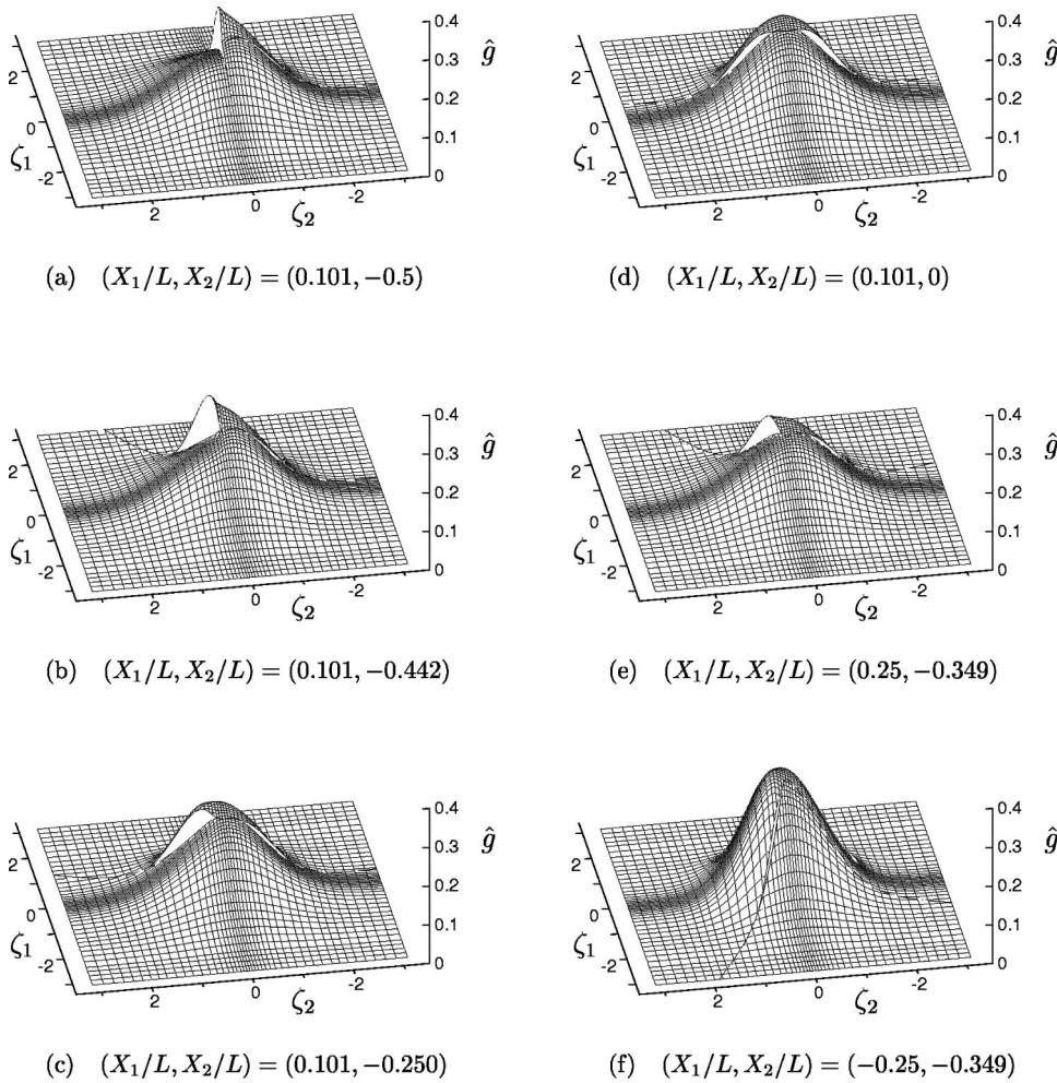
FIG. 16. Dimensionless marginal velocity distribution function \hat{g} [Eq. (28)] at six points in the gas for \text{Kn}=0.5 and T_2/T_1=2 . (a) (X_1/L, X_2/L) = (0.101, -0.5) , (b) (0.101, -0.442) , (c) (0.101, -0.250) , (d) (0.101, 0) , (e) (0.25, -0.349) , (f) (-0.25, -0.349) .
