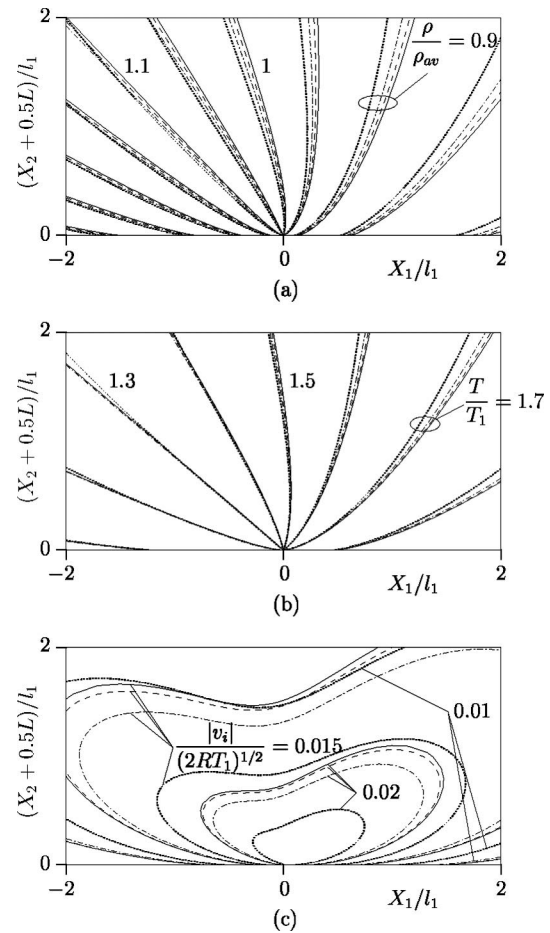
FIG. 14. Isolines of the density, temperature, and flow speed near the point of discontinuity at small Knudsen numbers for T_2/T_1 = 2 . (a) Density, (b) temperature, (c) flow speed. Here, the dotted line indicates the result for \text{Kn} = 0.05 , the dot-dashed line for \text{Kn} = 0.02 , the dashed line for \text{Kn} = 0.01 , and the solid line for \text{Kn} = 0.005 . The coordinates are normalized by the mean free path l_1 .
