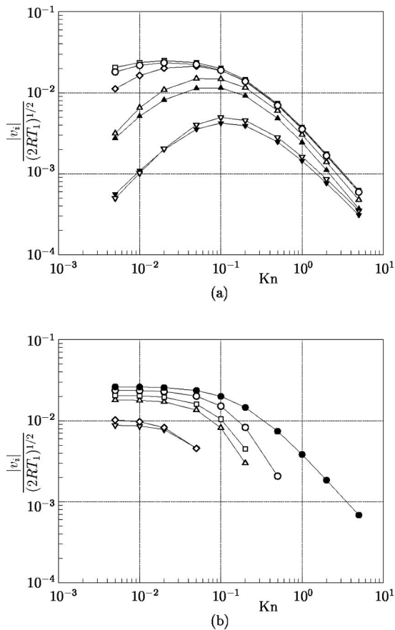
FIG. 13. Flow speed at various points in the gas vs the Knudsen number for T_2/T_1 = 2 . (a) The flow speed |v_i| at (X_1/L, X_2/L) = (0, -0.495) is shown by \circ , (0.005, -0.495) by \square , (0.02, -0.495) by \diamond , (0.05, -0.495) by \triangle , (-0.05, -0.495) by \blacktriangle , (-0.3, -0.4) by \blacktriangledown , and (0.3, -0.4) by \triangledown . (b) The flow speed |v_i| at (X_1/L, (X_2 + 0.5L)/L) = (0.5, 0.5) is shown by \circ , (1, 1) by \square , (5, 5) by \diamond , (2, 1) by \triangle , and (5, 1) by \triangledown ; the symbol \bullet indicates the maximum speed in the domain. In each figure, the same symbols are joined by straight lines.
