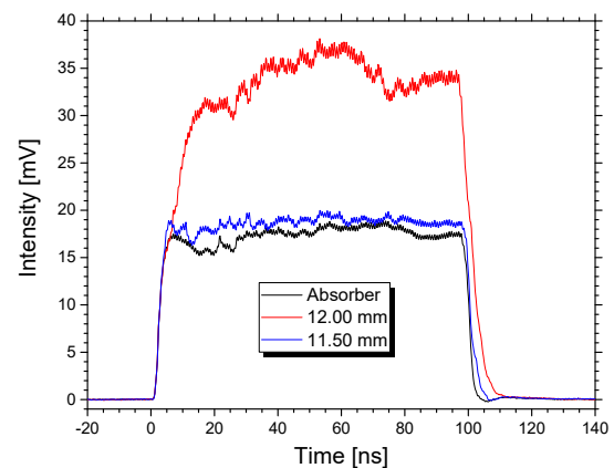
Fig. 2. Measured temporal evolution of the horizontal component of CTR micropulse power.
