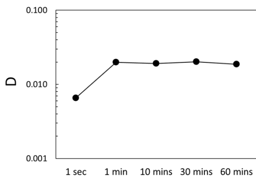
Fig. 1. Distribution coefficient (D) of Ca isotope on various extraction time using DC18C6 crown-ether: Preliminary.
