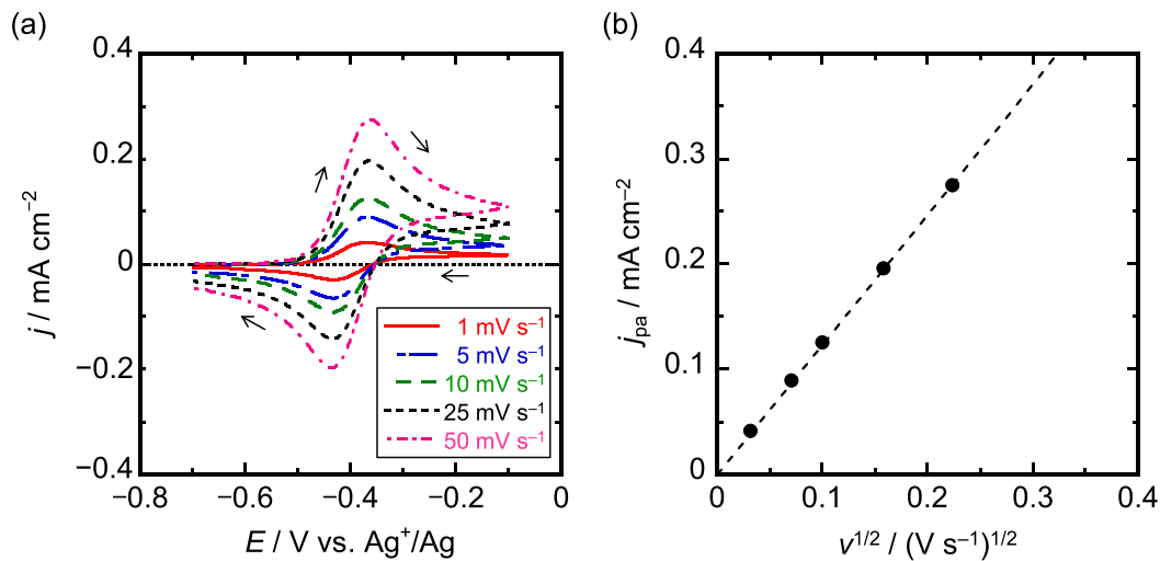
Figure S16 (a) Cyclic voltammograms of a platinum disk in Na[FSA]-[C 3 C 1 pyrr][FSA] ionic liquid ( x(\text{Na[FSA]}) = 0.20 ) containing 10 \text{mmol dm}^{-3} ferrocene. Scan rates: 1–50 \text{mV s}^{-1} . Temperature: 298 K. (b) Correlation plots of current densities and the square root of scan rates.
