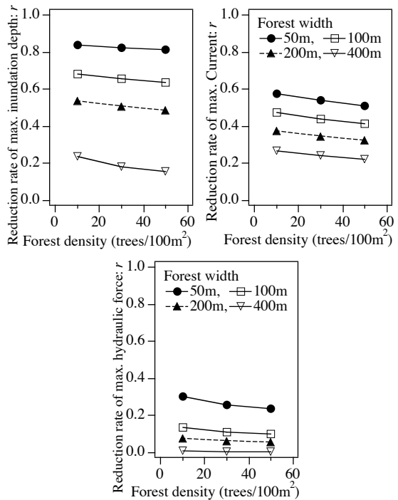
Fig. 7 Effect of forest density to tsunami reduction (Tsunami period 10 min)
