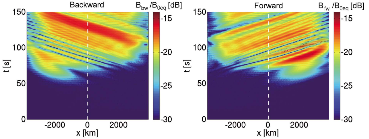
Figure 1. Spatial and temporal evolution of the wave amplitudes of the backward and forward propagating EMIC waves.
