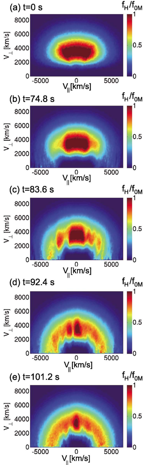
Figure 3. Velocity distribution functions f_H(v_{\parallel}, v_{\perp}) of energetic protons at (a) t = 0 s, (b) t = 74.8 s, (c) t = 83.6 s, (d) t = 92.4 s, and (e) t = 101.2 s normalized by the maximum value of the initial velocity distribution function f_{0M} .
