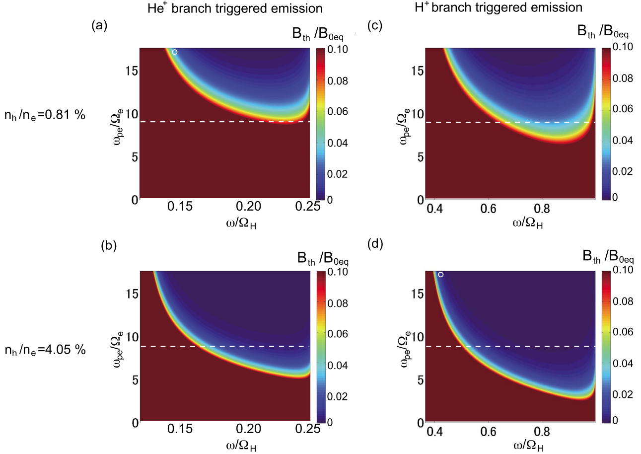
Figure 5. Theoretical thresholds of nonlinear wave growth as functions of frequency f and electron density n_e for \text{He}^+ branch triggered emissions with densities of energetic protons (a) n_h/n_e = 0.81\% and (b) n_h/n_e = 4.05\% , and those for \text{H}^+ branch triggered emissions with densities of energetic protons (c) n_h/n_e = 0.81\% and (d) n_h/n_e = 4.05\% . The ambient magnetic field, the proton cyclotron frequency, and the electron cyclotron frequency at the equator are B_{0eq} = 243 nT, \Omega_H = 23.2 rad/s, and \Omega_e = 4.27 \times 10^4 rad/s, respectively. The dashed white lines indicate an electron density 50/cc corresponding to the possible plasmopause. The white circles in Figures 5a and 5d indicate the input parameters used in the present \text{He}^+ branch simulation and the previous \text{H}^+ branch simulation [Shoji and Omura, 2011], respectively.
