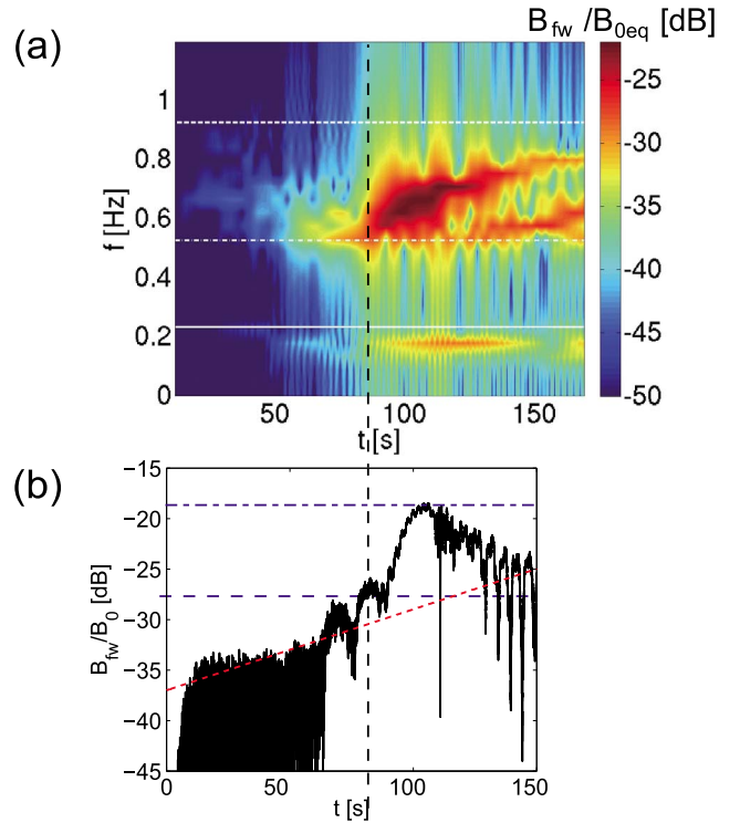
Figure 2. (a) Dynamic spectra of the magnetic field of forward propagating waves. The solid, dash-dotted, and dashed white lines show the cyclotron frequency of O + , the theoretical frequency of the triggered waves, and the cyclotron frequency of He + , respectively. (b) Time evolution of the wave amplitude at the equator in log scale. The dashed red line shows the linear growth rate of the EMIC wave. The dashed and dash-dotted blue lines show the theoretical threshold B_w = 0.48 nT and the saturation level B_{sat} = 3.5 nT of the EMIC triggered emission, respectively. The dashed black line shows the time when the nonlinear wave growth starts ( t \sim 85 s).
