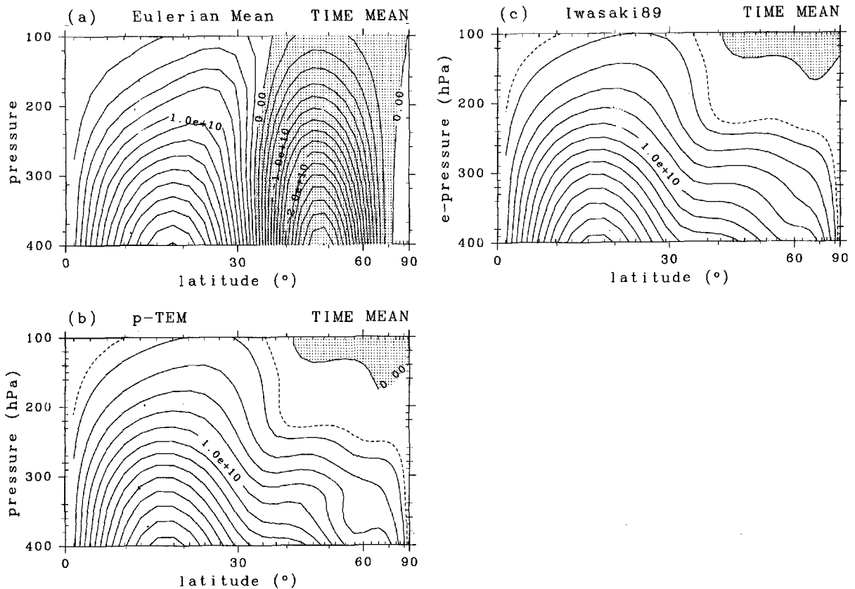
Fig. 11 Climatology of the mass-weighted streamfunction of mean meridional circulation. (a) Eulerian mean with p coordinate. (b) Transformed Eulerian mean with p coordinate. (c) Iwasaki (1989)'s formulation of transformed Eulerian mean with p_e coordinate. Contour interval of solid curves is 2.0 \times 10^9 \text{ kg s}^{-1} , and that of broken curves is 1.0 \times 10^9 \text{ kg s}^{-1} . Negative (indirect) regions are shaded.
