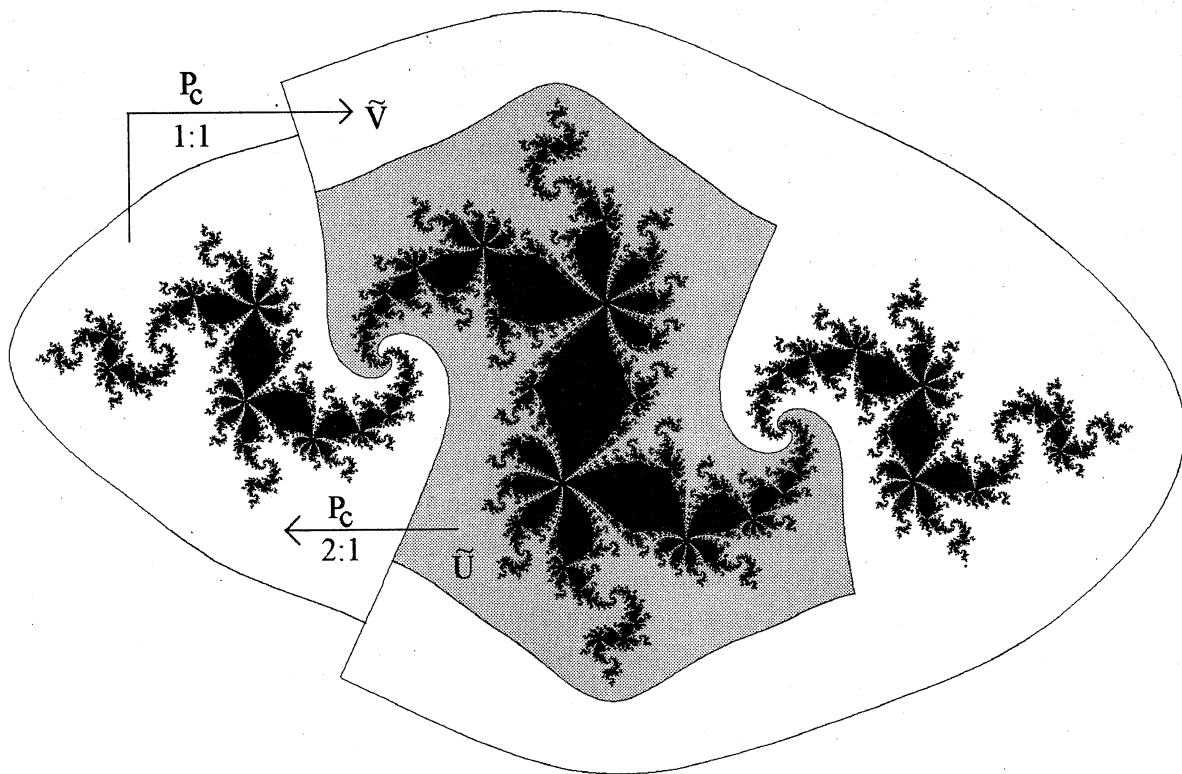
Figure 1: An example of a simple renormalization of \beta -type.
