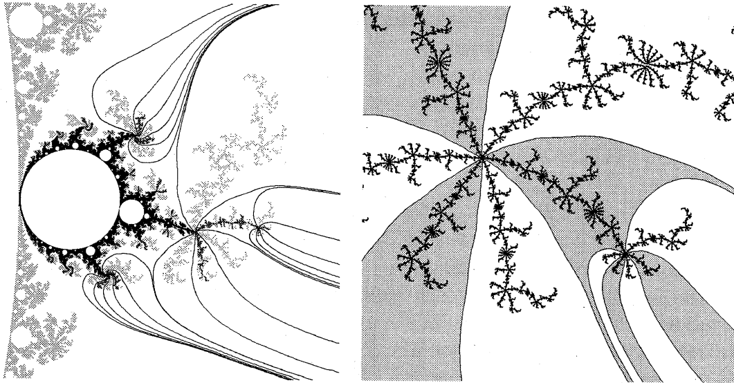
Figure 3: Left: the renormalization locus C_{p,q}^n in M_{p/q} , displayed for n = 2 and p/q = 1/3 : the entire Mandelbrot set is shown in light grey; the crossed 2-renormalization locus is shown in dark grey, and the simple 6-renormalization locus is shown in black. Right: some dynamic rays corresponding to parameter rays bounding the renormalization locus.
