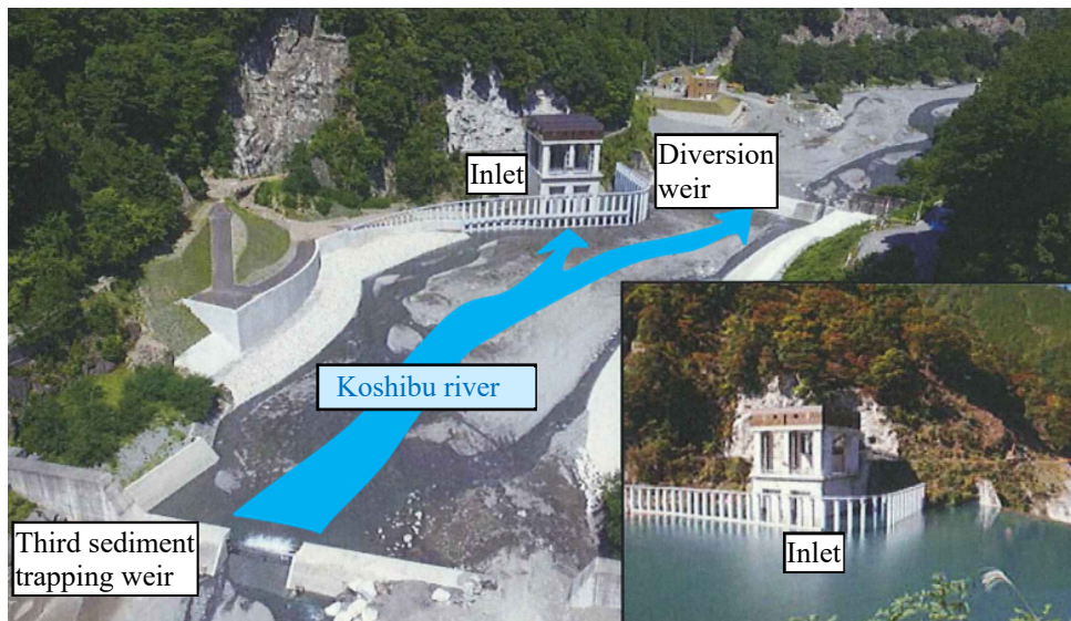
Figure 1: Sediment bypass facility of Koshibu Dam (source: Tenryu River Dam Integrated Management Office)
