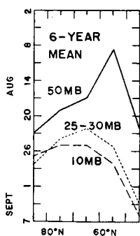
Fig. 4. The date of fall reversal of the stratospheric circulations averaged over 6 years from 1957 through 1962.
