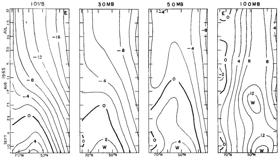
Fig. 2. Meridional and time sections of the zonal winds averaged longitudinally.
