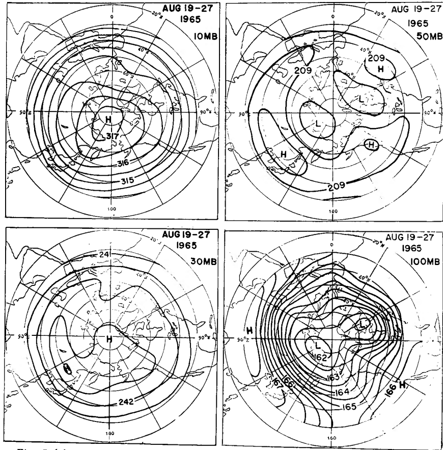
Fig. 5 (e). 9-day mean maps for Aug. 19-27, 1965.
