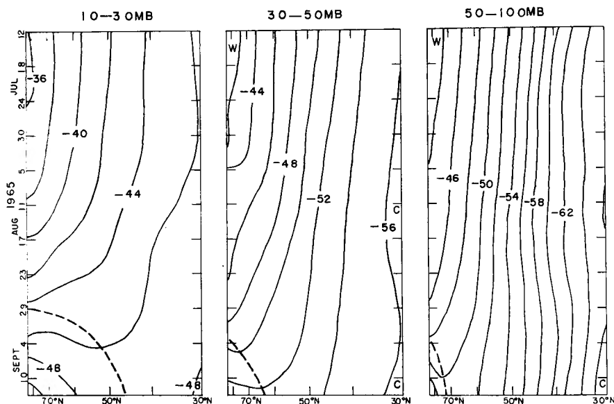
Fig. 6. Meridional and time sections of longitudinally, averaged temperature. The unit is °C. Cosine-scale is used in the abscissa.
