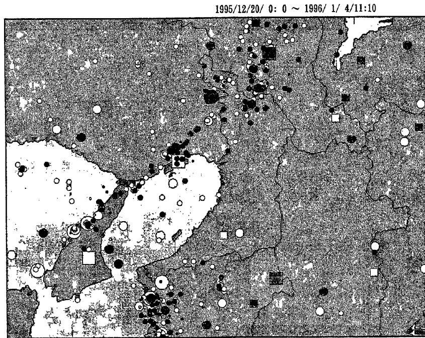
Fig. 4. An example of real time information of seismicity around the source region including neighboring areas, which has been sending to local self governing bodies in Kinki district by means of a personal computer transmission. The original is displayed by color.
