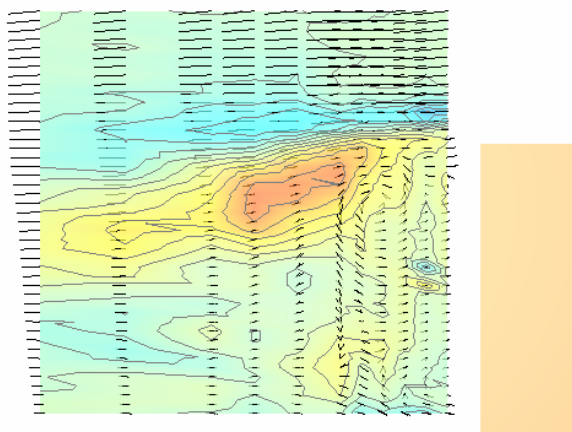
Figure 9 Longitudinal vorticity contour and velocity vector of time averaged flow in parallel section at y/D=0.5 .
