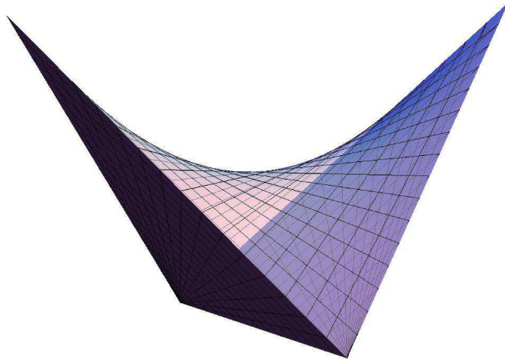
Figure 2. The set \mathcal{E}_3
