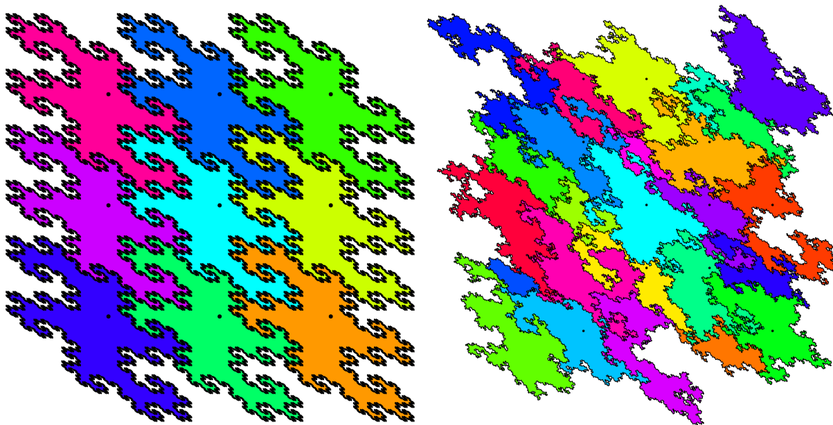
Figure 16. Two patches of tiles induced by SRS tiles: the left figure shows the tiling associated with the parameter \mathbf{r} = (1/2, 1) . It is an affine image of the tiling induced by the CNS defined by X^2 + 2X + 2 . The central tile is Knuth's twin dragon. The right patch corresponds to the parameter \mathbf{r} = (2/3, 1) . It can also be regarded as the Brunotte tiling associated with the non-monic expanding polynomial 2X^2 + 3X + 3 .
