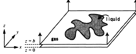
Figure 4.1: Hele-Shaw cell
