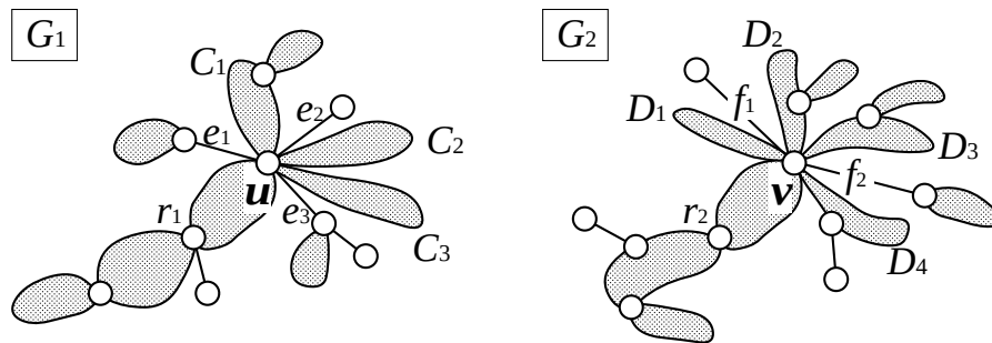
Figure 2. Computation of MCS_c(G_1(u), G_2(v)) .
