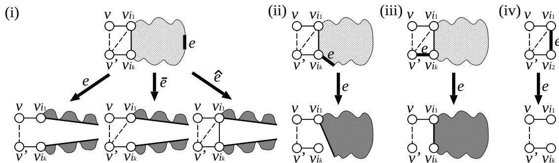
Figure 7. Types and subcases of blades, where two other subcases for (ii) and another subcase (i.e., \{v', v_{i_1}\} remains) for (iii) and (iv) are omitted.
