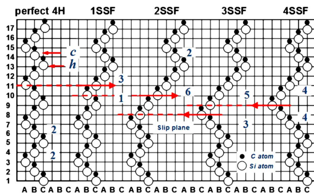
FIG. 4. (Color online) Schematic of the stacking sequences of the Shockley type SFs viewed from the [11\bar{2}0] direction. Stacking sequences are illustrated in terms of the ABC and Zhdanov's notations.
