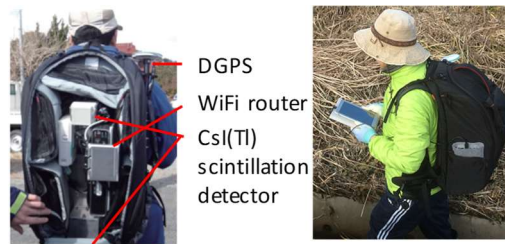
Fig 1. KURAMA-II system
