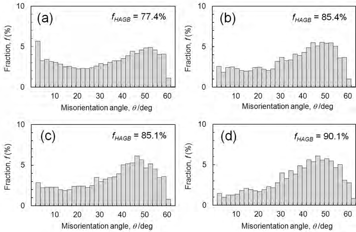
Figure 2.8 Misorientation angle distributions of the low-C (UFG-FC1) steel cold-rolled by 91% reduction and annealed at (a) 620 °C, (b) 635 °C, (c) 655 °C and (d) 680 °C for 120 s followed by water-cooling. f_{HAGB} indicates the fraction of high angle grain boundaries (HAGBs) in the microstructures.
