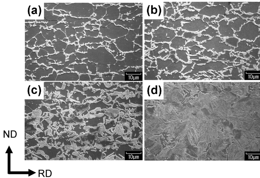
Figure 3.11 SEM microstructures of (a) the as-received DP590 steel, and the specimens after annealing at (b) 750 °C, (c) 800 °C and (d) 850 °C of the DP590 steel. The microstructures in (a, b, c) were dual-phase (DP) ones composed of ferrite and martensite, and the microstructure of (d) was 95% martensite. Observed from TD.
