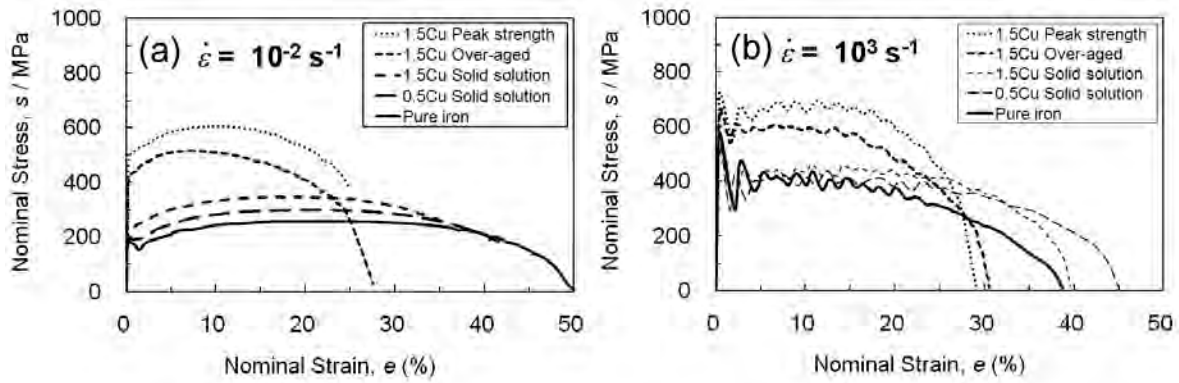
Figure 3.15 Stress-strain curves of the pure iron, Fe-0.5 mass% Cu alloy and Fe-1.5 mass% Cu alloy. For Fe-1.5 mass% Cu alloy, data of the specimens precipitation-treated at the peak-strength condition, and at the over-aged condition are shown. The strain rates are (a) 10^{-2} \text{ s}^{-1} and (b) 10^3 \text{ s}^{-1} .
