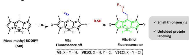
Fig. 1 Substituted meso -vinyl BODIPY (VBs) as thiol-selective fluorogenic probes for small thiol sensing and unfolded proteins labelling, prepared from meso -methyl-BODIPY (MB).
