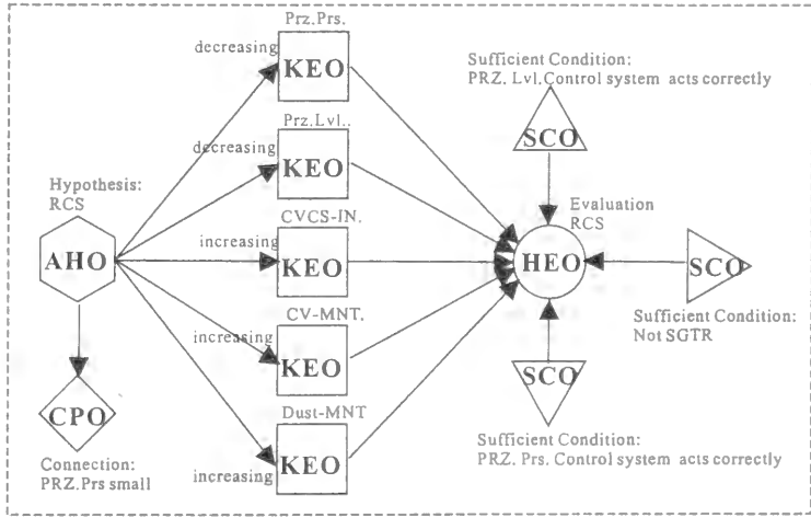
Figure 3.10: Modeling methods of the knowledge about "RCS leakage"
