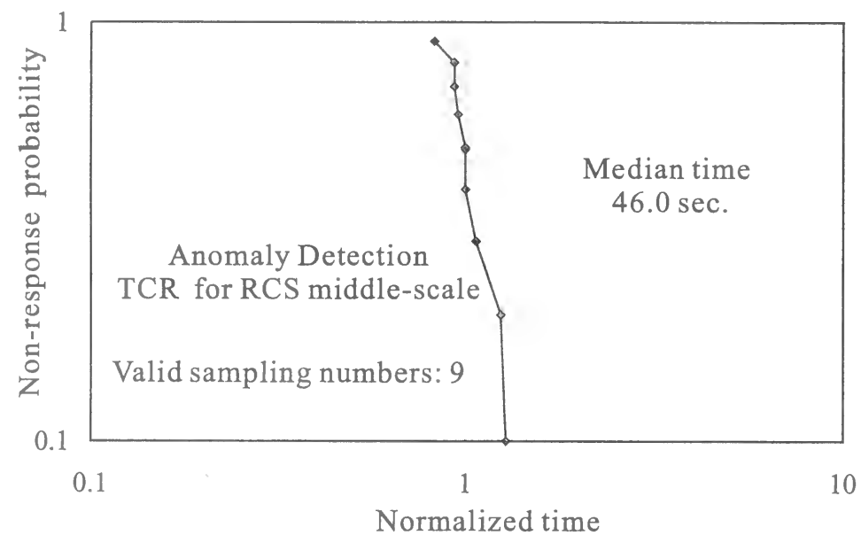
Figure F.3: TCR curves for detecting "RCS leakage middle-scale"
