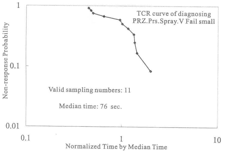
Figure F.17: TCR curves for diagnosing “PRZ. Spray V. Fail small”
