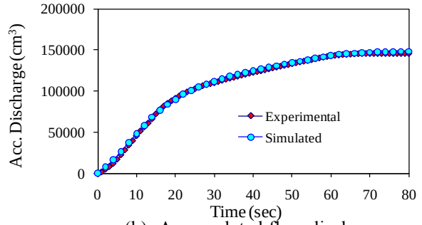
(b) Accumulated flow discharge
