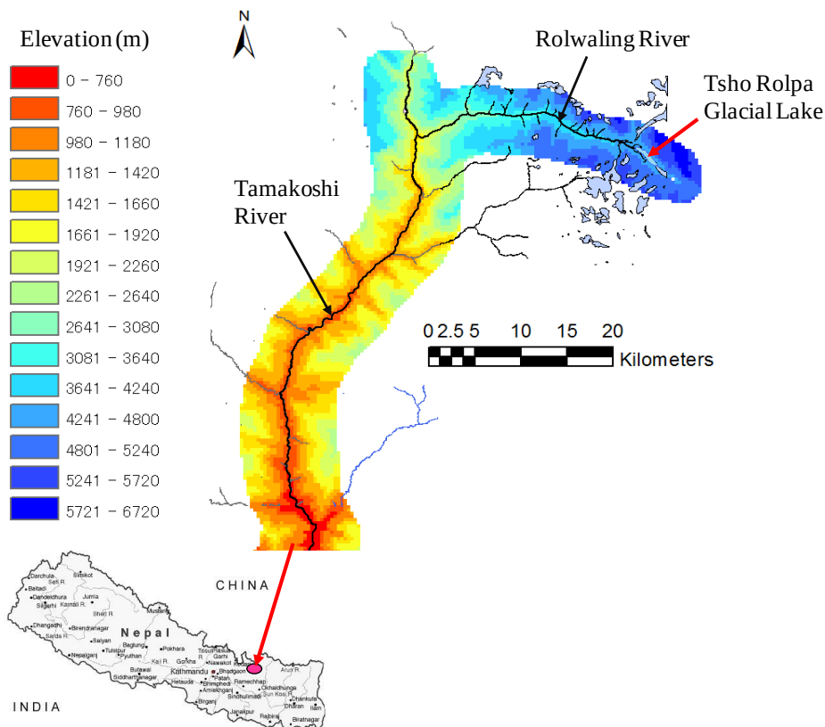
Fig. 1 Location of Tsho Rolpa Glacial Lake and digital elevation model of river valley
