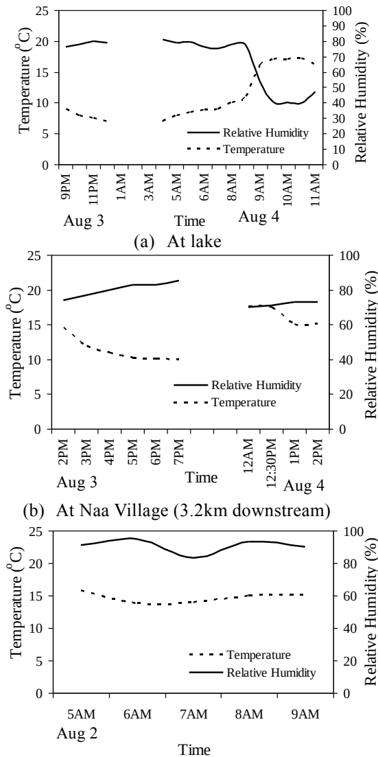
(c) At Donggang Village (18.8km downstream) Fig. 2 Measured temperatures and relative humidity at the lake and downstream villages (in 2010)
