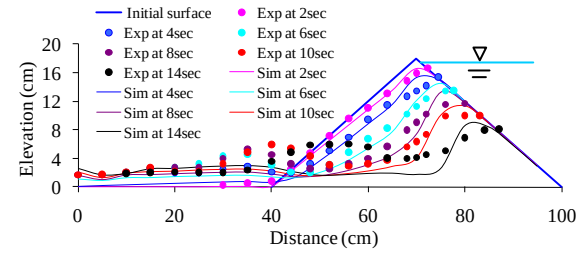
Fig. 42 Temporal variations of dam surface due to erosion, Case-III, time t=0 sec is the starting time of erosion, 5.54% initial moisture content
