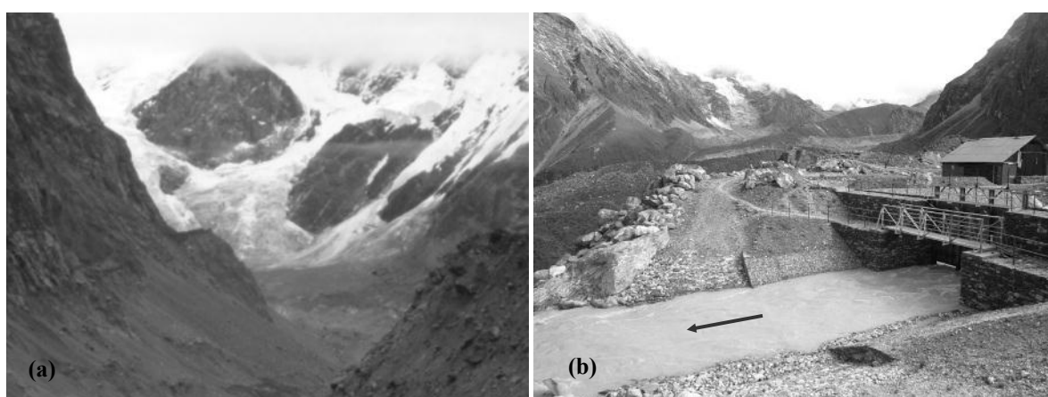
Fig. 9 (a) Trakarding glacier at the upstream end of the lake, (b) Lake outlet open channel constructed at the end of moraine dam (Photograph by: Badri Bhakta Shrestha, August 2010)
