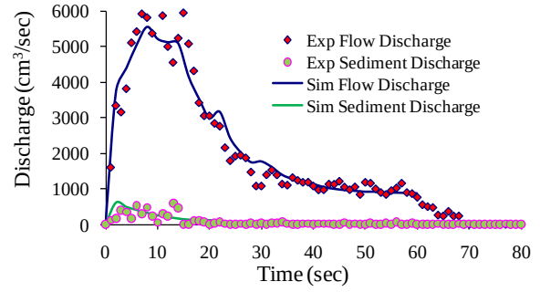
(a) Outflow discharge
