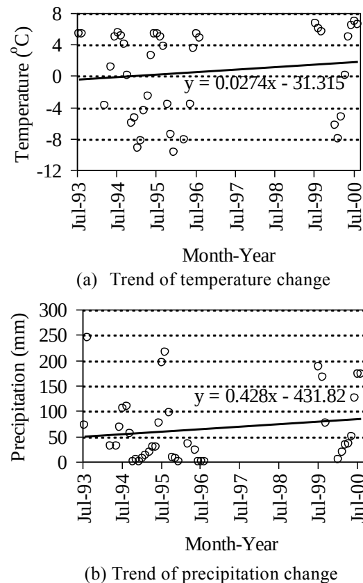
(b) Trend of precipitation change Fig. 4 Trend of temperature and precipitation changes at Tsho Rolpa Glacial Lake (Data Source: Department of Hydrology and Metrology (DHM), Nepal)
