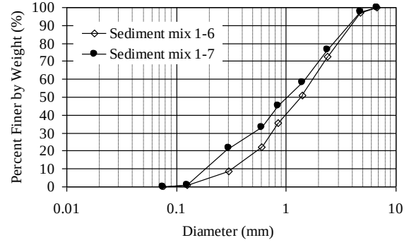
Fig. 28 Particle size distribution of bed sediment
