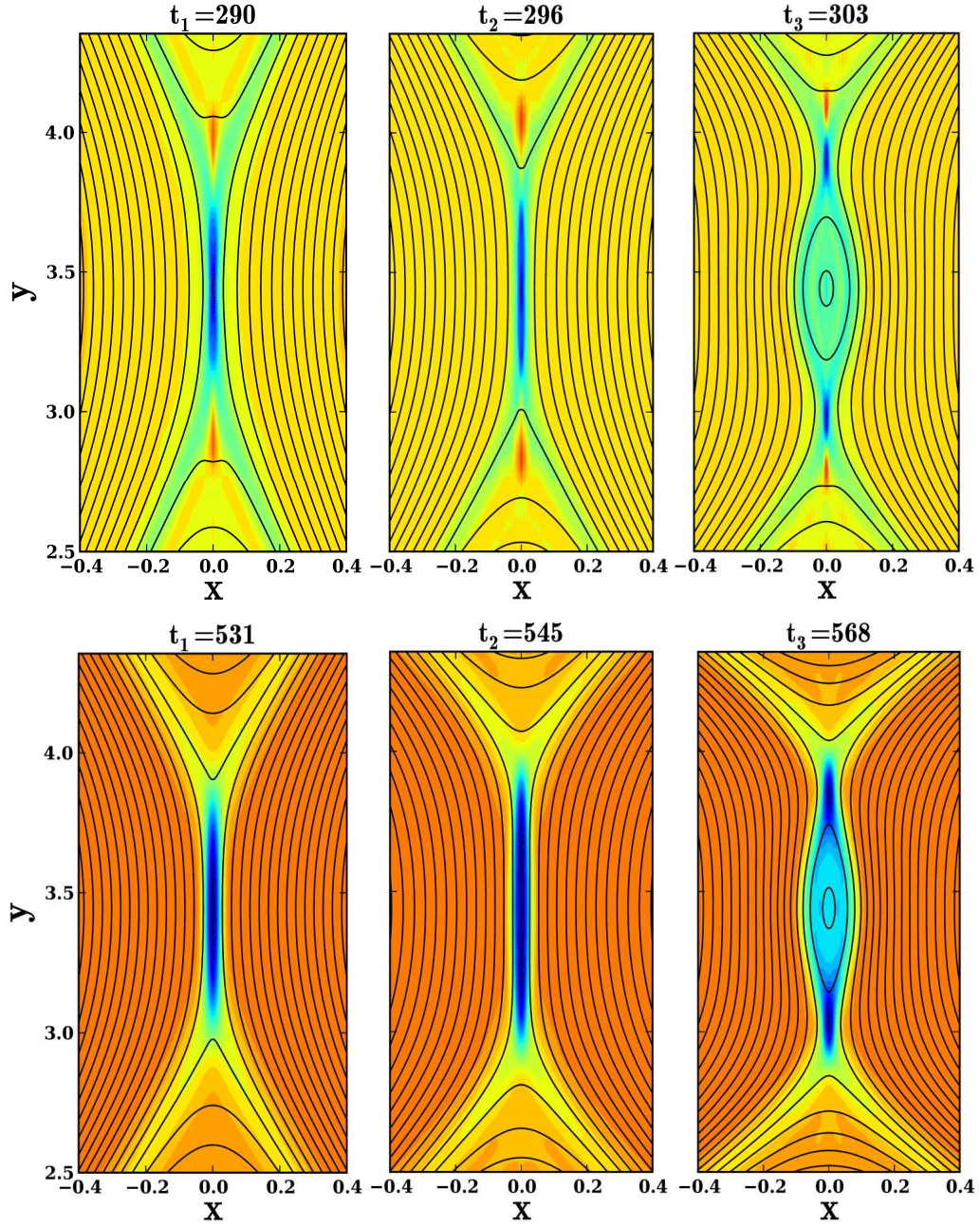
Figure 4.12: 2D contour plots of the current, merged with the magnetic flux lines, during the nonlinear evolution of Figure. 4.11. The upper panel represents the case of P_r = 0 and lower panel P_r = 10 .
