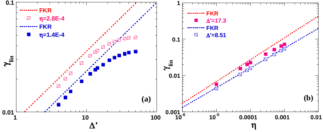
Figure 3.2: Scaling of the linear growth rate verses (a) instability parameter \Delta' for two cases of resistivities, and verses (b) resistivity \eta for two fixed values of \Delta' . The dashed lines, represents the theoretical scalings of the linear growth rate as predicted by FKR.
