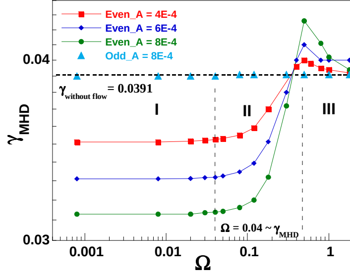
Figure 5.8: Linear growth rates of the tearing mode verses the frequency of radial even-parity dynamic flow for different amplitudes (solid curves). The triangular marks represent the case with odd-parity flow. The horizontal dashed line references the growth rate in the case without flow; vertical dashed lines partition the parameter region with different physical dependence. Simulation parameters are \eta = 2.8 \times 10^{-4} , \Delta' = 17.3 and k_y^{DF} = 2.75 .
