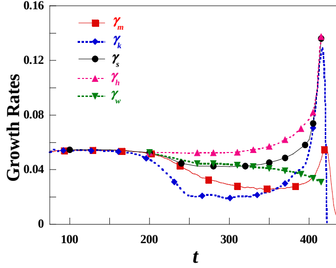
Figure 4.5: Time history of the secondary growth rates of perturbation energy due to zonal current, current peaking and current broadening (represented by \gamma_s , \gamma_h and \gamma_w respectively) along with the growth rates of the mean square electrostatic and magnetic potential ( \gamma_m and \gamma_k ). The simulation parameters are the same as in Figure 4.2.
