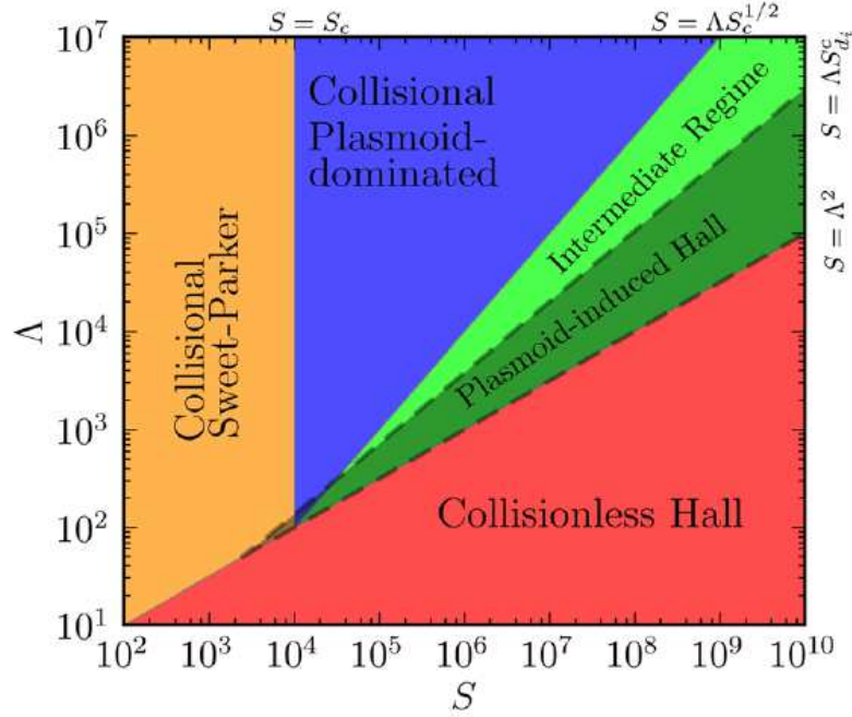
Figure 1.16: Phase diagram of magnetic reconnection showing five phases in the parameter space of S and \Lambda = L/d_i , where d_i is the ion inertial length .
