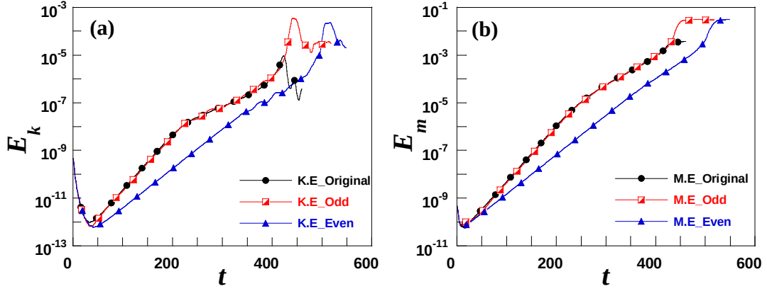
Figure 5.4: Time history of mean square perturbed electrostatic potential E_k = \langle \phi^2 \rangle / 2 (a) and magnetic potential E_m = \langle \psi^2 \rangle / 2 (b) for Even/Odd dynamic flows. The simulation parameters are \eta = 1.4 \times 10^{-4} , A = 8 \times 10^{-4} and \Omega = 0.08 .
