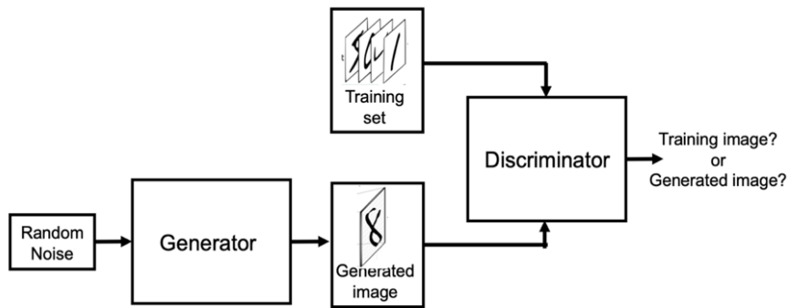
Fig. 7. The primary configuration of GAN ([3])
