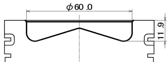
Fig.2 Combustion chamber shape
