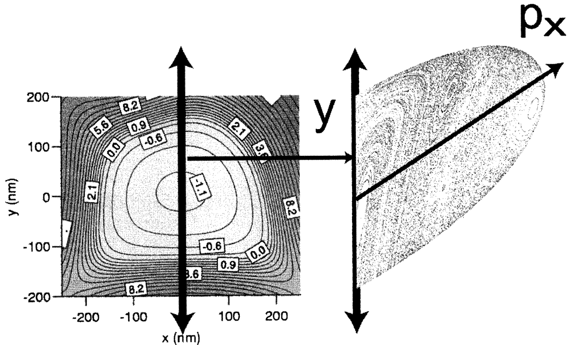
Figure 1 Effective 2D potential contour V(x,y) of quantum dot. Potential contours labeled in Ry (1 Ry \approx 5.8 meV), Fermi surface at V=0 . Schematic shows definition of Poincaré surface of section (SOS), chosen as line that bisects dot (typically x=0 ) and x -component of momentum as
