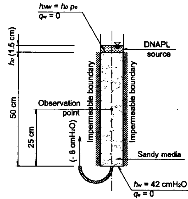
Fig. 6 The apparatus for multiphase column test
