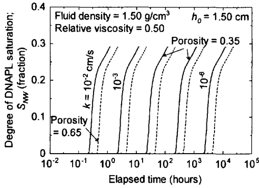
Fig. 12 Influence of the saturated hydraulic conductivity on the migration process
