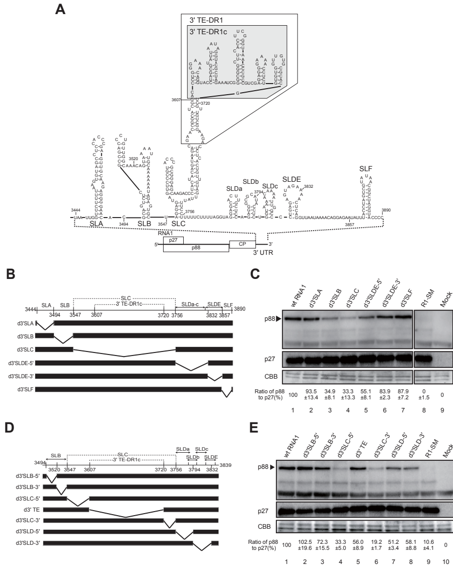
Fig. I-1. Identification of the regions required for -1 PRF in RCNMV RNA1. (A) Schematic diagram of RCNMV RNA1 and the secondary structure predicted in the 3' UTR (Iwakawa et al., 2007). Numbers indicate nucleotide positions in RCNMV RNA1. (B and D) Schematic representation of deleted regions in the 3' UTR of RCNMV RNA1. Boldface lines indicate the virus-derived sequences with the nucleotide numbers at the 5' and 3' ends. Bent lines indicate the deleted regions. (C and E) The effects of deletions in the 3' UTR of RCNMV RNA1 on -1 PRF. RNA1 and its mutants were incubated in BYL for 4 h, and the accumulated levels of p27 and p88 were analyzed by western blotting using an anti-p27 antiserum. Coomassie brilliant blue-stained cellular proteins are shown below the western blottings as a loading control. The accumulated levels of both p27 and p88 were quantified with the Image Gauge program (Fuji Photo Film, Tokyo, Japan), respectively. The ratios of p88 to p27, calculated as a percentage relative to wt RNA1 (set to 100), are shown below the EtBr-stained rRNA with standard errors of the mean from at least three independent experiments.
