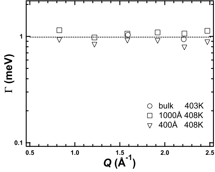
Figure 4.12: Q dependence of relaxation rate \Gamma of the fast process for bulk ( \circ ), 1000 \text{\AA} ( \square ), 400 \text{\AA} ( \nabla ).
