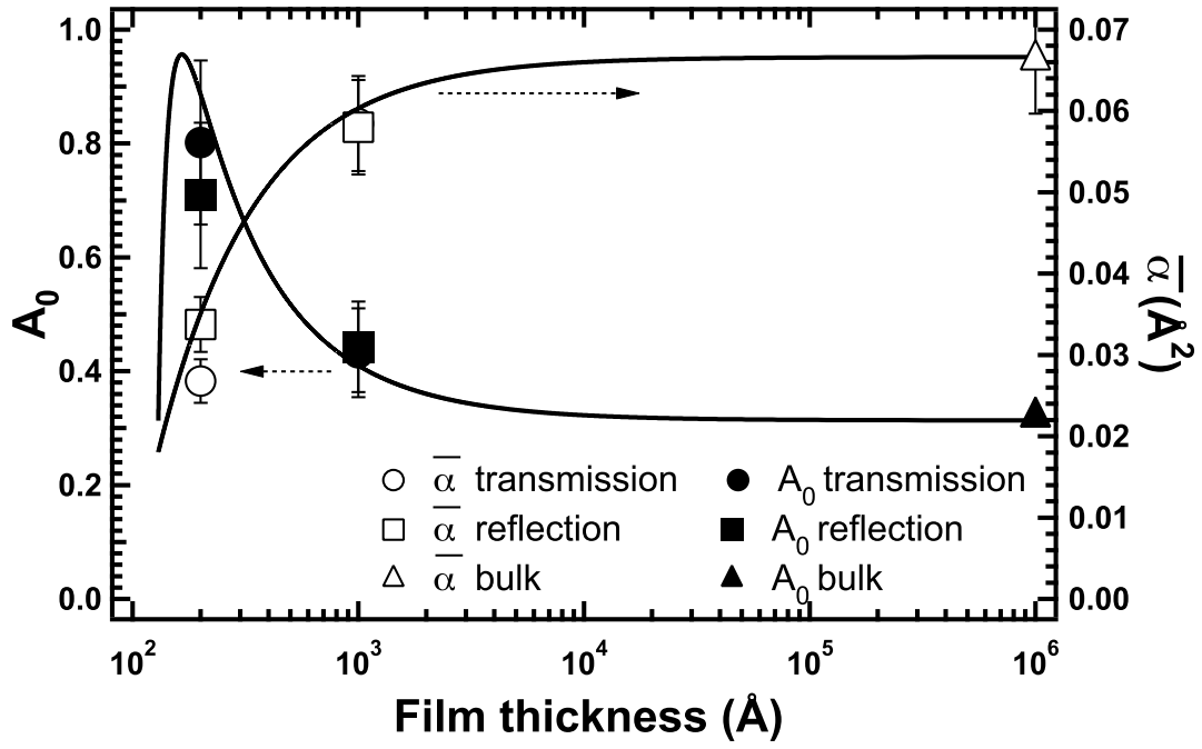
Figure 6.10: Thickness dependence of mean square displacement \bar{\alpha} in transmission (○) and reflection (□) geometries, and non-Gaussian parameter A_0 in transmission (●) and reflection (■) geometries at 230 K. \bar{\alpha} (△) and A_0 (▲) for bulk are also shown in figure. Solid curves are the results of fit using bi-layer model.
