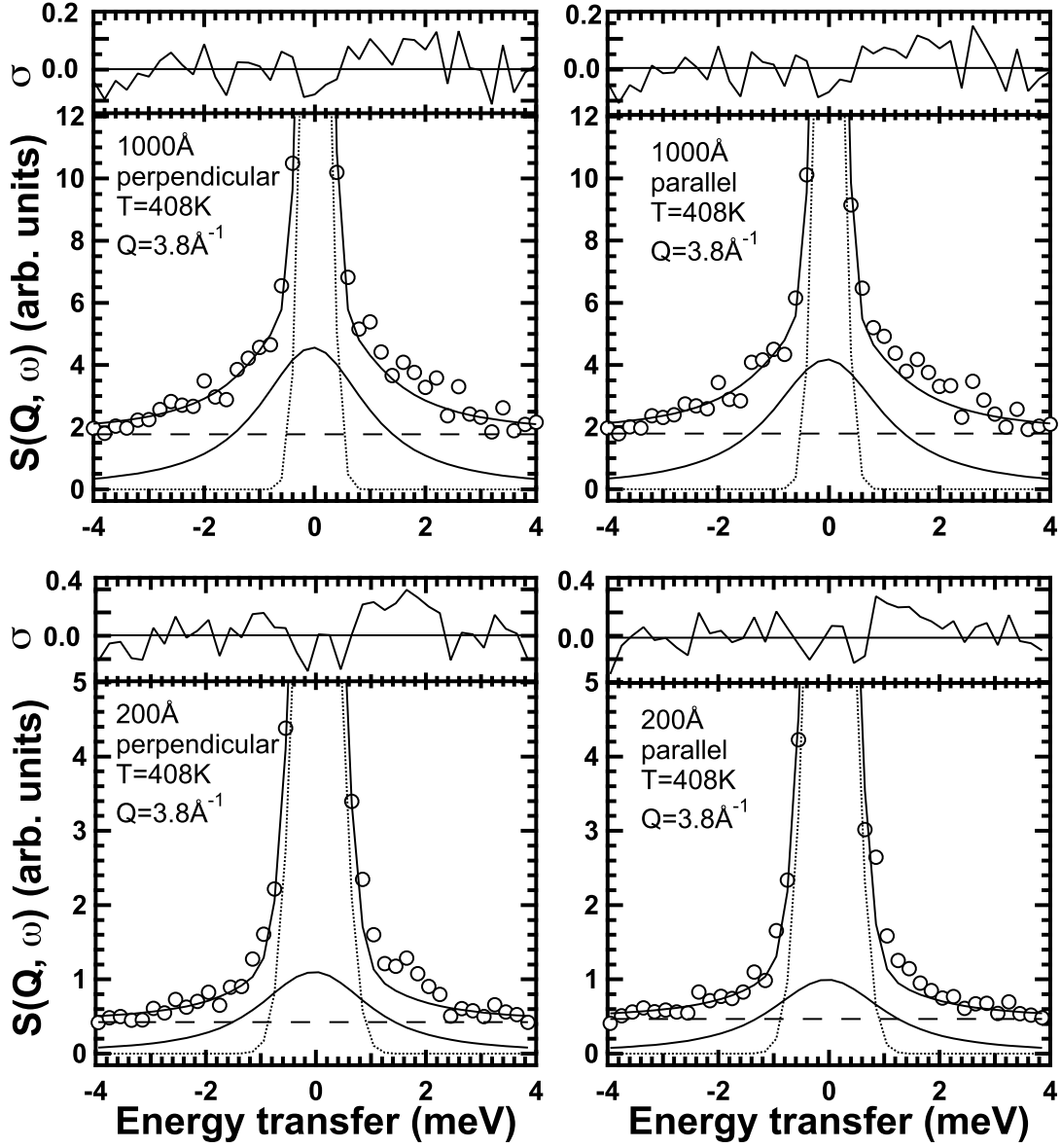
Figure 6.5: Results of curve fits to S(Q, \omega) of 1000 and 200 Å PS thin films at 408 K at Q=3.8 \text{ Å}^{-1} for parallel and perpendicular geometries. ( \cdots ): elastic component, ( — ): quasielastic Lorentzian and ( - - ): flat background.
