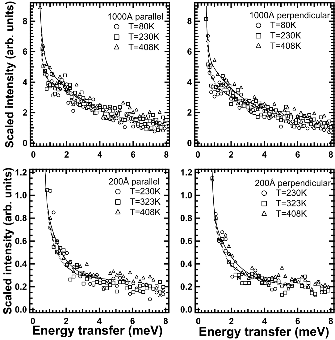
Figure 6.3: Bose-scaled dynamic scattering law S(Q, \omega) of 1000 and 200 Å PS thin films at various temperatures at Q=3.8 \text{ Å}^{-1} in perpendicular and parallel geometries after correcting for Debye-Waller factor. Solid lines were drawn by eye for the spectra at 408 K for both 1000 and 200 Å films. Dashed lines were also drawn by eye for the spectra at 80 K for 1000 Å film and at 230 K for 200 Å film in the low energy region below 2 meV
