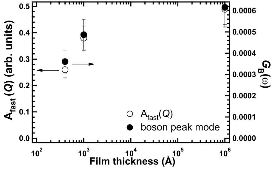
Figure 4.13: Thickness dependence of fraction of the fast process A_{\text{fast}}(Q) ( \circ ) and density of phonon states of the Boson peak mode G_B(\omega) ( \bullet ).
