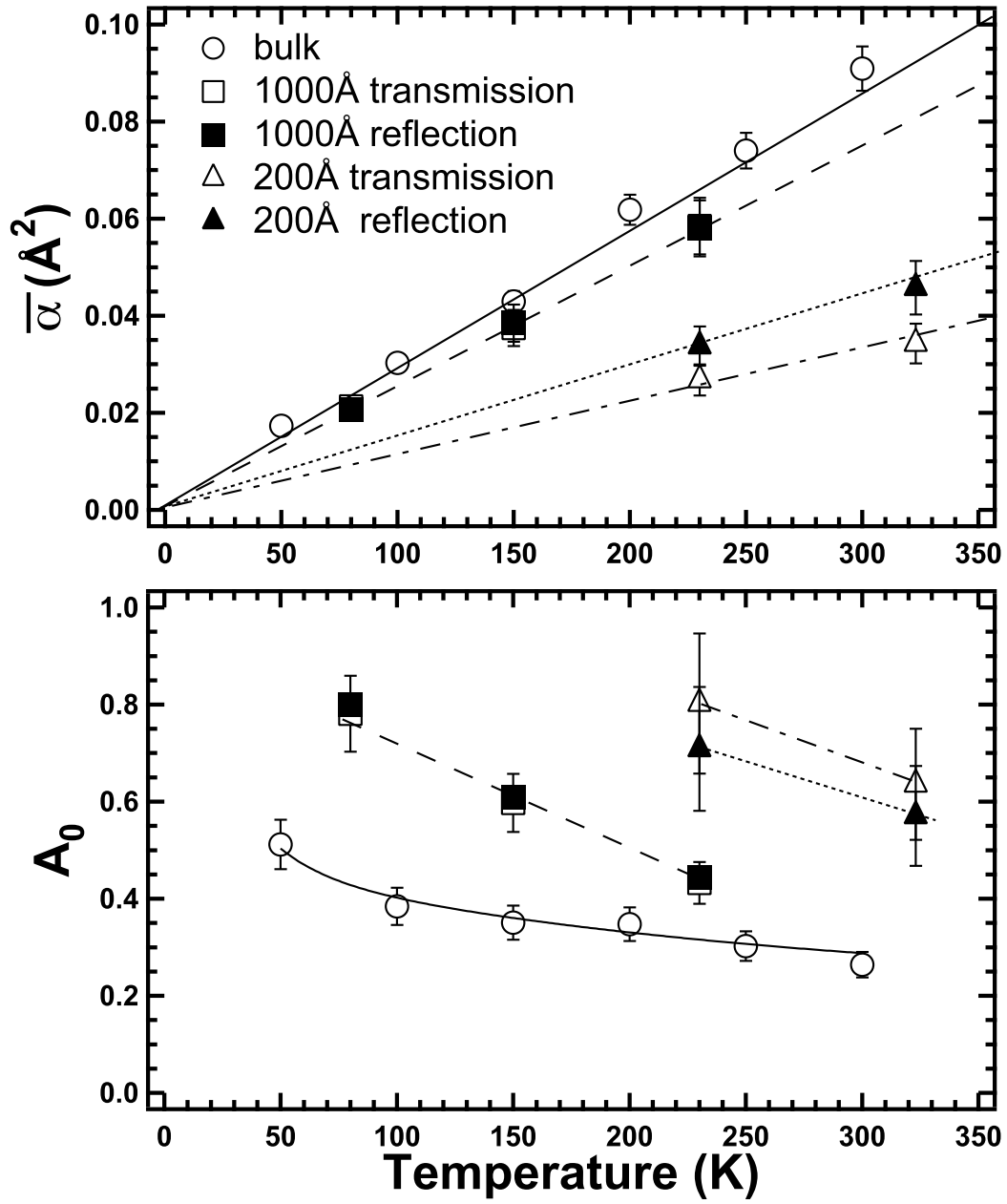
Figure 6.8: Temperature dependence of mean square displacement \overline{\alpha} and non-Gaussian parameter A_0 for bulk ( \circ ), 1000 \text{\AA} film in transmission ( \square ) and reflection ( \blacksquare ) geometries, and 200 \text{\AA} film in transmission ( \triangle ) and reflection ( \blacktriangle ) geometries.
