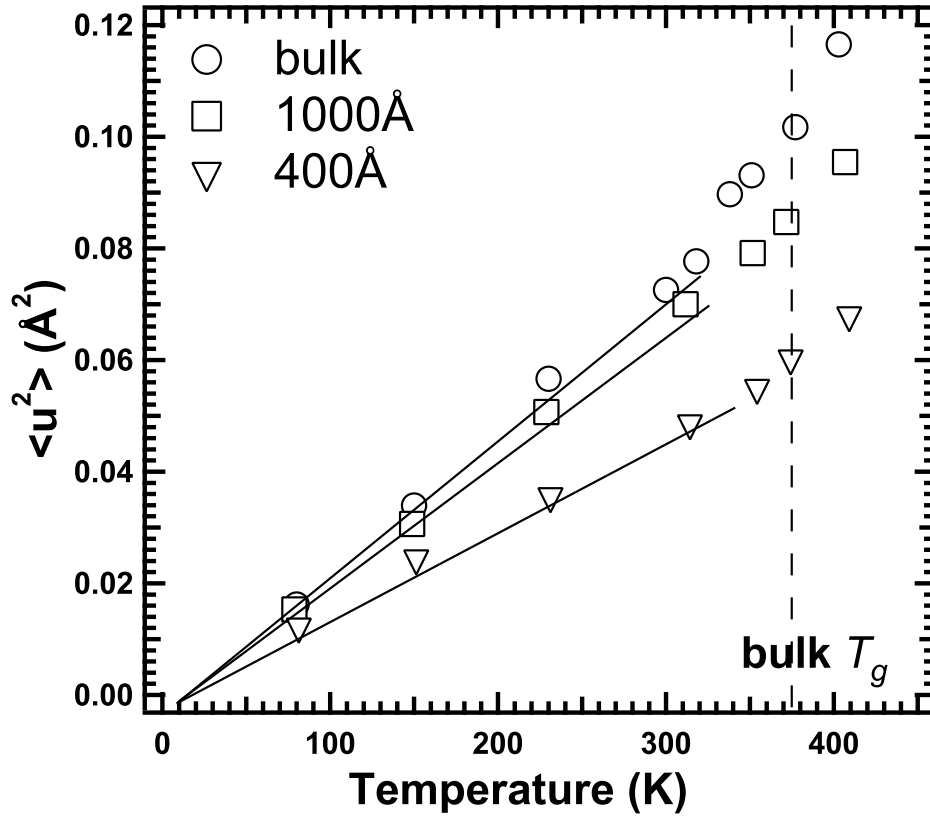
Figure 4.3: Temperature dependence of mean square displacement \langle u^2 \rangle : bulk( \circ ), 1000 Å ( \square ), and 400 Å ( \nabla ). Dashed line shows bulk glass transition temperature T_g .
