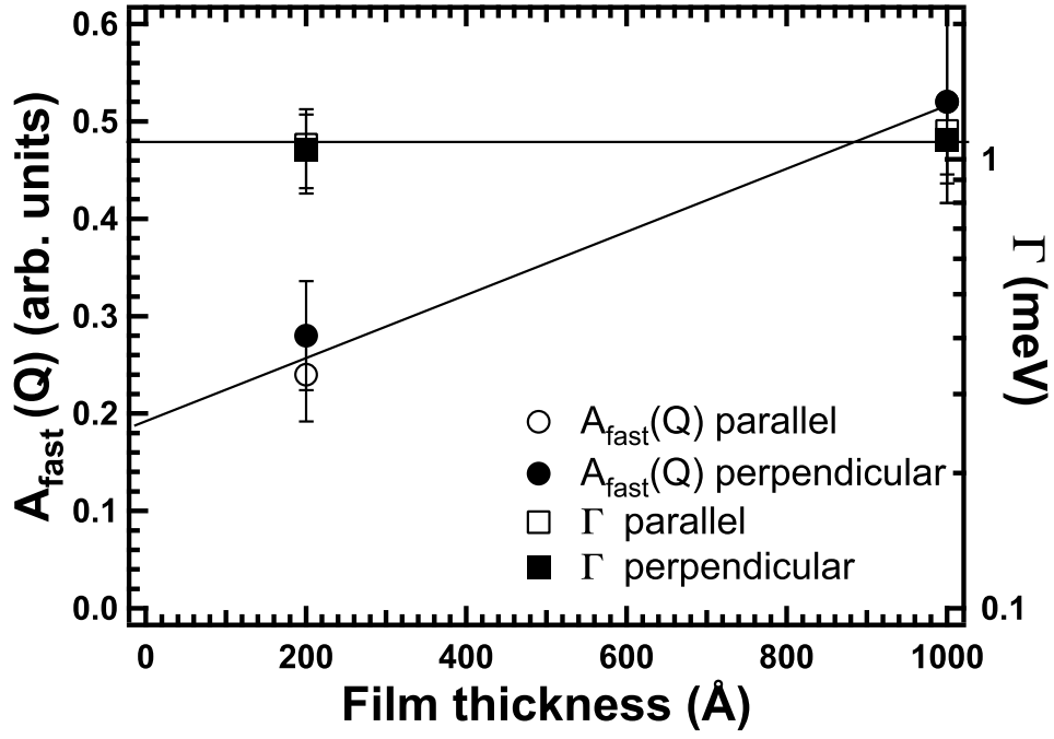
Figure 6.6: Film thickness dependence of relaxation rate \Gamma and fraction A_{fast}(Q) of the fast process at 408 K for parallel and perpendicular geometries. Parallel (○, □) and perpendicular (●, ■). Square and circle symbols correspond to \Gamma and A_{fast}(Q) , respectively.
