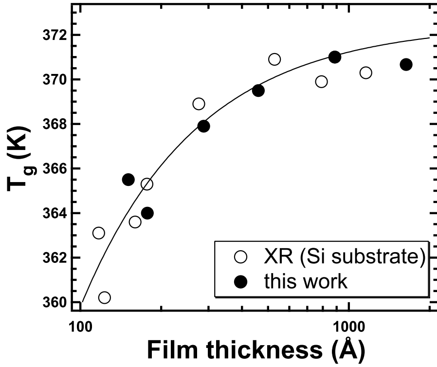
Figure 3.3: Thickness dependence of T_g obtained from this work (●) and the data obtained from XR (○) and solid line is the result of fit with two-layer model.
