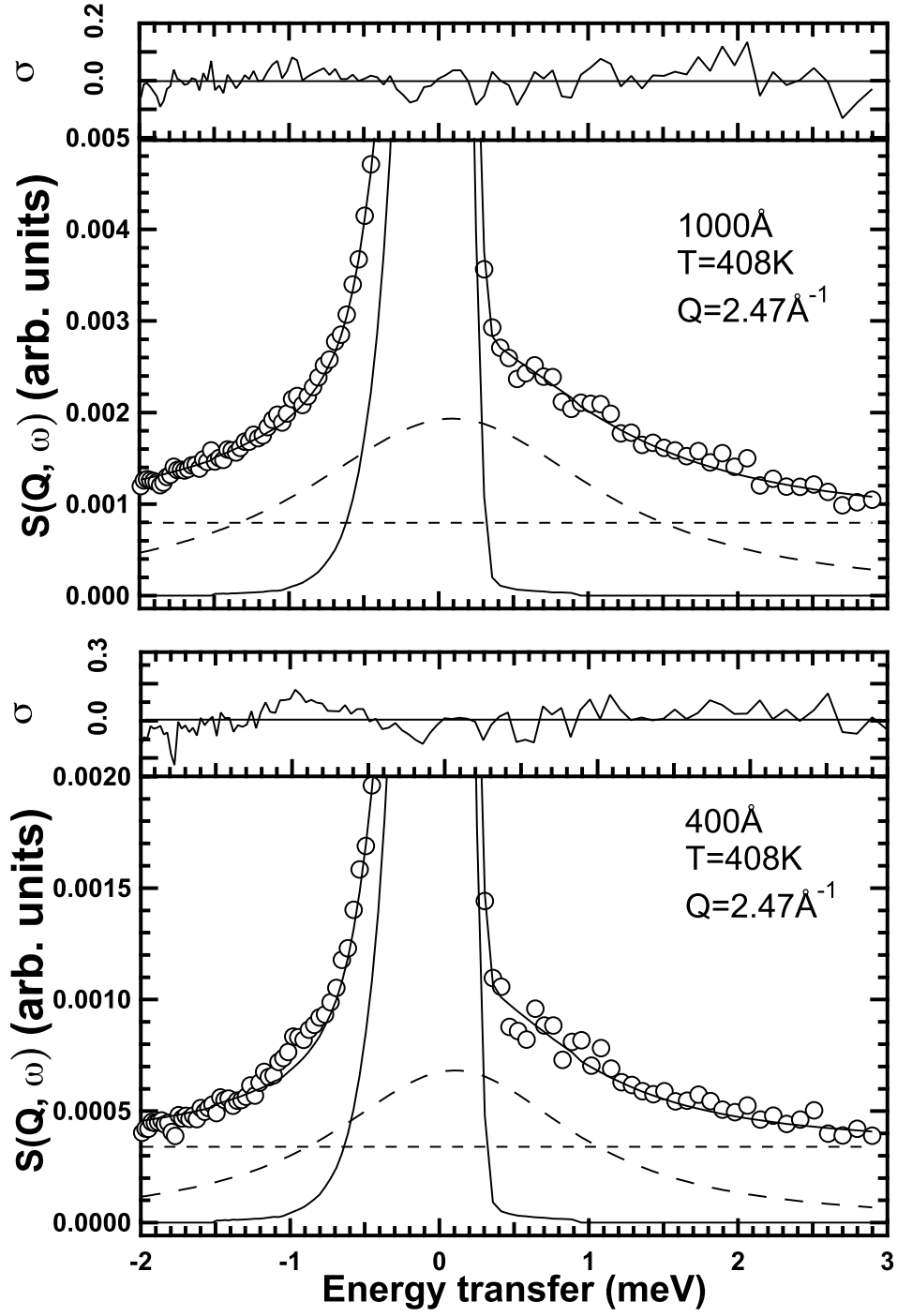
Figure 4.10: Results of curve fitting to the LAM-40 spectra of 1000 \text{ \AA} and 400 \text{ \AA} thin films at T = 408 \text{ K} and Q = 2.47 \text{ \AA}^{-1} . (—): elastic component, (---): quasielastic Lorentzian and (- - -): flat background.
