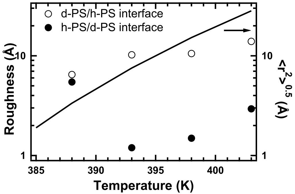
Figure 8.5: Temperature dependence of roughness at d-PS/h-PS interface ( \circ ) and h-PS/d-PS interface ( \bullet ) and solid line shows the temperature dependence of root of mean square displacement estimated from reptation.
