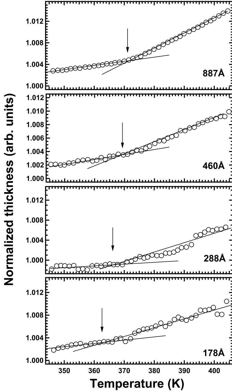
Figure 3.2: Temperature dependence of film thickness normalized by thickness at room temperature, which is shown in each box and the arrows indicate T_g .
