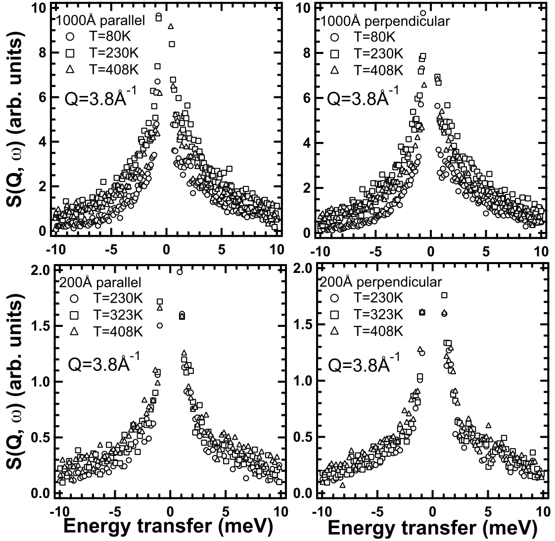
Figure 6.2: Dynamic scattering law S(Q, \omega) of 1000 and 200 Å PS thin films at various temperatures at Q = 3.8 \text{ \AA}^{-1} in perpendicular and parallel geometries.
