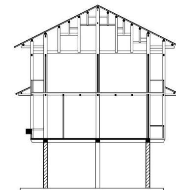
SECTION
