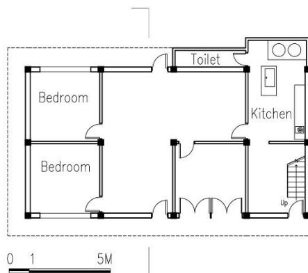
1F PLAN
