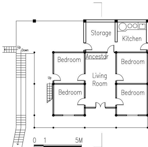
1F PLAN
