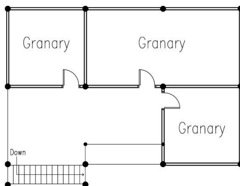
2F PLAN
