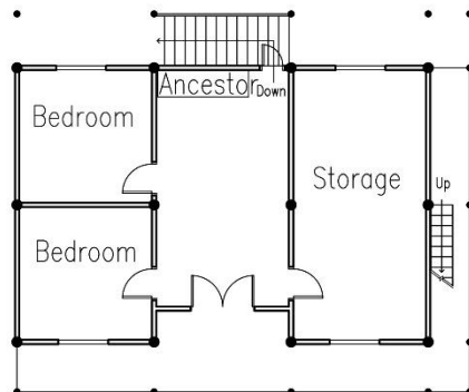
2F PLAN
