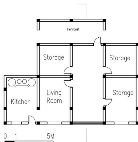
1F PLAN
