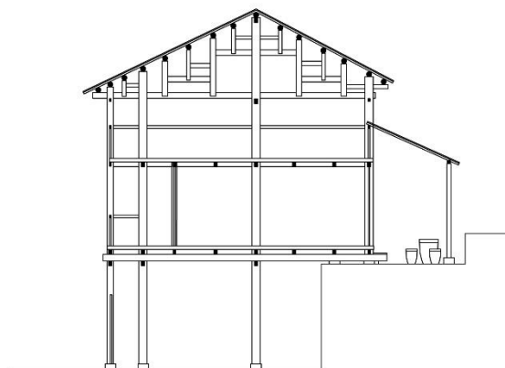
SECTION
