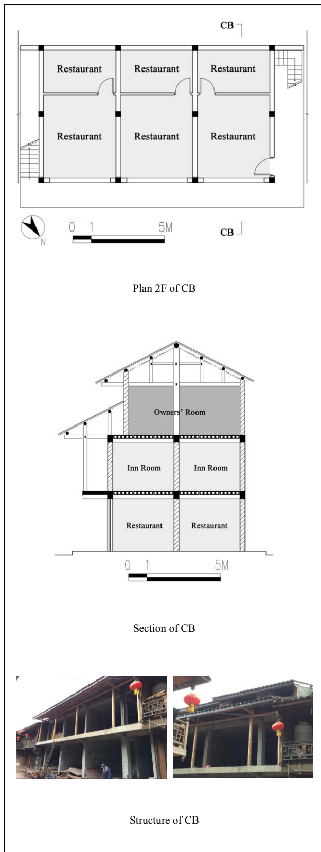
Figure 3. 8 Building samples of confined-brick (CB) and reinforced concrete buildings (RC)
