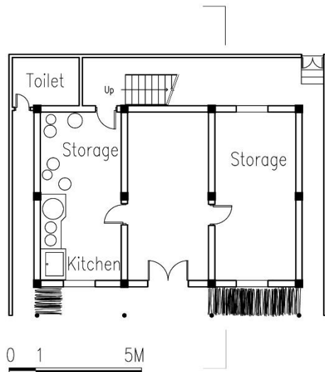
1F PLAN
