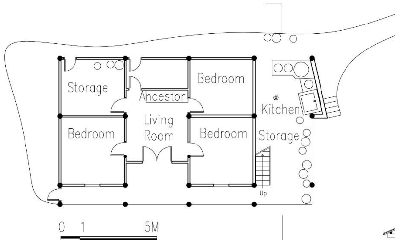
1F PLAN
