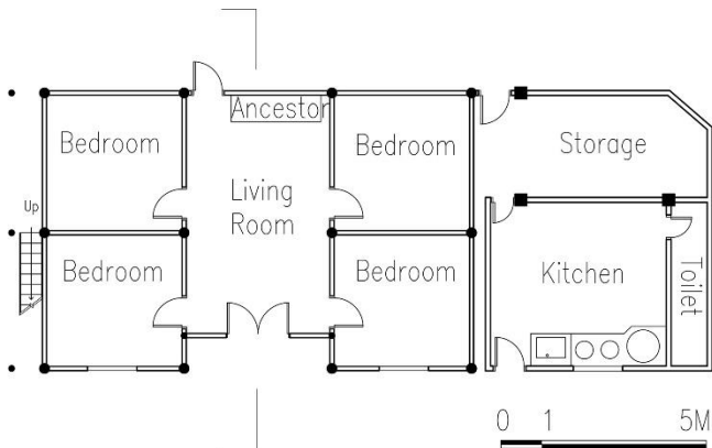
1F PLAN
