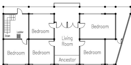
2F PLAN
