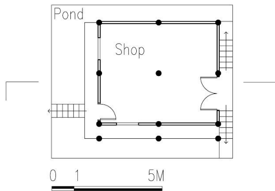
1F PLAN
