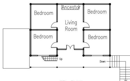
2F PLAN
