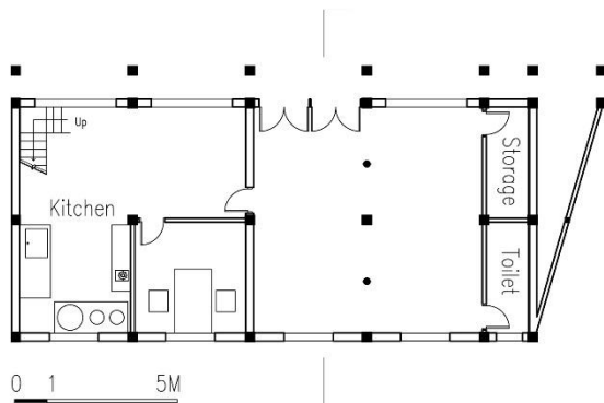
1F PLAN
