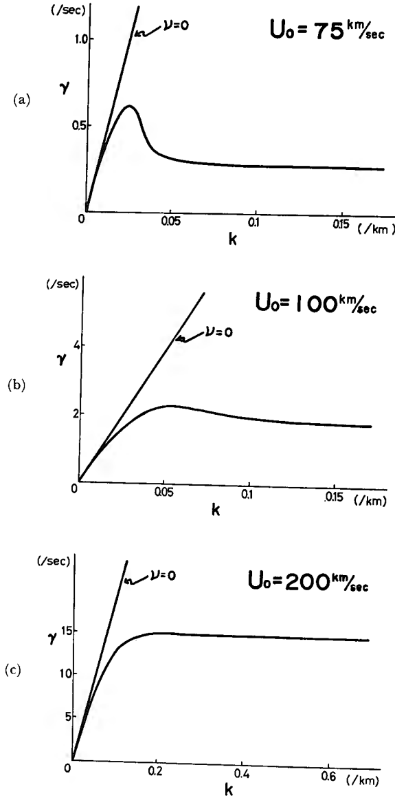
Fig. 2. The growth rate \gamma as a function of wave number k , taking B_0=20\gamma , N_0=50\text{ cm}^{-3} and T_0=5\times 10^5\text{ K} . (a), (b) and (c) refer to U_0=75 , 100 and 200 km/sec respectively. The straight line corresponds to the case of zero Larmor radius.
