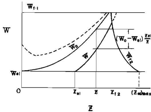
Fig. 10 Relationship between W and z , ( W_{el} = W_e ).
