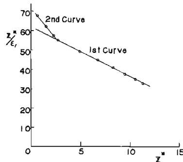
Fig. 9 Experimental linear relationship of z/\gamma_p \sim z constructed from the 1st and 2nd stress-strain curves at plastic state shown in Fig. 1
