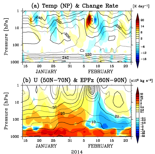
Fig. 1 Time-height cross section of (a) the North Pole temperature (contour, interval: 10 K) and its change rate (color, unit: K day -1 ), (b) zonal-mean zonal wind averaged over latitudes from 50°N to 70°N (contour, interval: 5 m s -1 ) and the vertical component of E-P flux averaged northward of 60°N (color, unit: 10 5 kg s -2 ). The shading shows the region of easterly winds.
