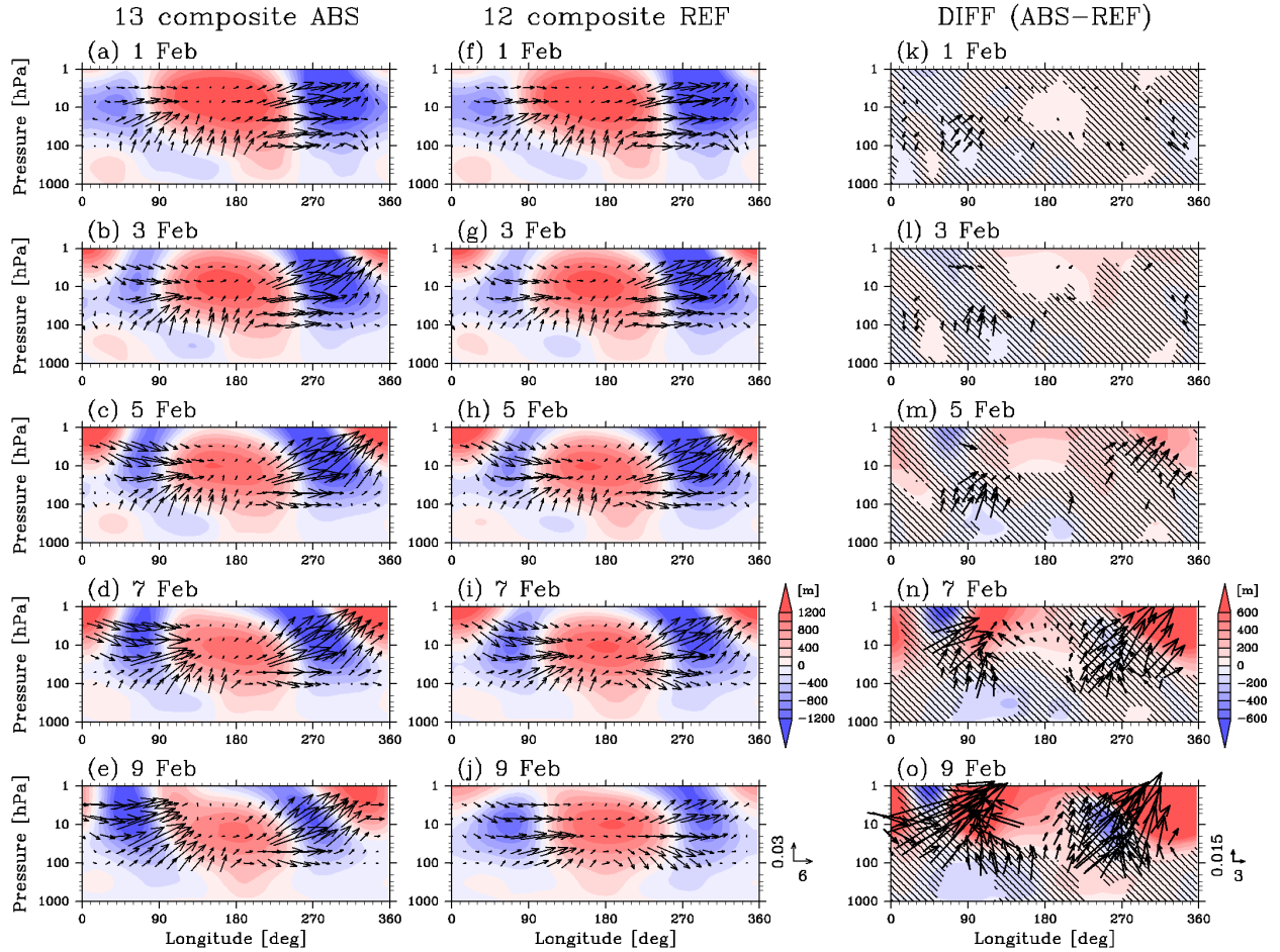
Fig. 6 (a-j) Longitude-height cross section of eddy geopotential height (color, unit: gpm) and vertical and zonal component of the 3-D Plumb flux (arrows, unit: \text{Pa}^{-0.5} \text{ m s}^{-2} , scaled by the inverse the square root of the pressure) averaged northward of 60^\circ\text{N} for the composites of ABS and REF groups (left and center columns). (k-o) Same as (a-j), except for the difference (ABS - REF) of the geopotential height. The region whose difference is insignificant at 99% confidence (estimated by Welch's t -test) is shaded. The difference of the Plumb flux is plotted when its vertical component is significant at 95% confidence. Each panel from top to bottom shows a daily-mean field for 1, 3, 5, 7 and 9 Feb., respectively.
