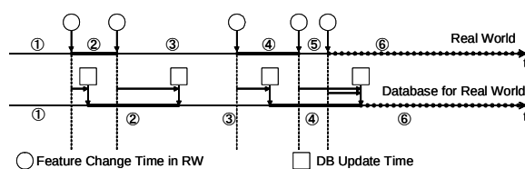
Fig.1 Feature Changes on Database
