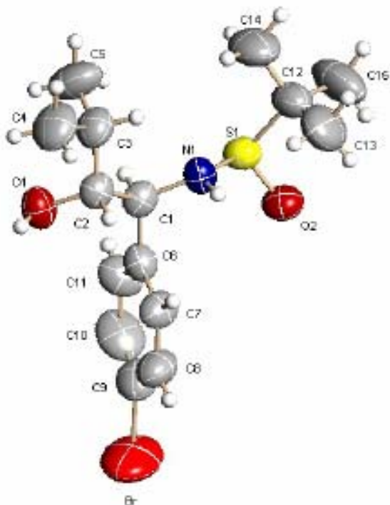
Figure 2 X-ray Crystal Structure of Cross-coupling Product 6b
