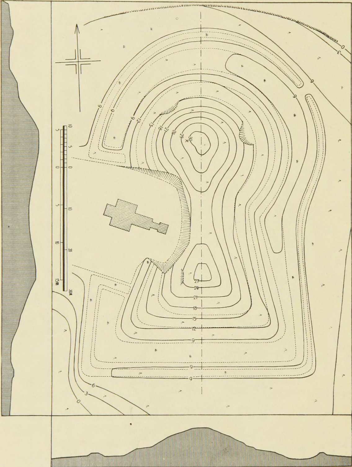
Fig. 2. Plan and Sections of the Tenjin-yama Tomb at Keisen-mura
