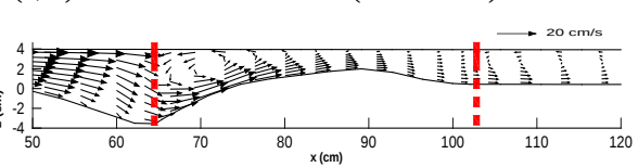
Fig.16b Longitudinal-section velocity vectors (u,w) at y=72.0\text{cm} – Case 3 (simulation)
