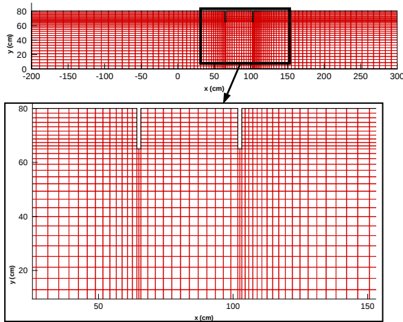
Fig.4a Grid of computed area for impermeable groins with details of groins field
