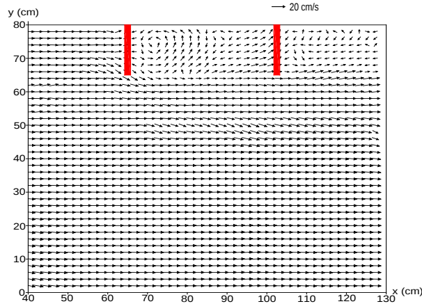
Fig.7a Flow velocity (u,v) at water surface by PIV – Impermeable groins (experiment) – Case 1
