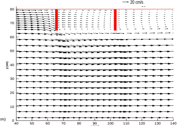
Fig.9b Flow velocity (u,v) at water surface – Bandal-like structures (simulation) – Case 3
