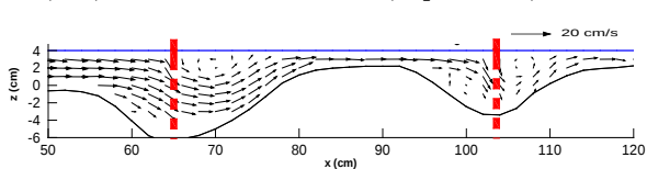
Fig.16a Longitudinal-section velocity vectors (u,w) at y=72.0\text{cm} – Case 3 (experiment)
