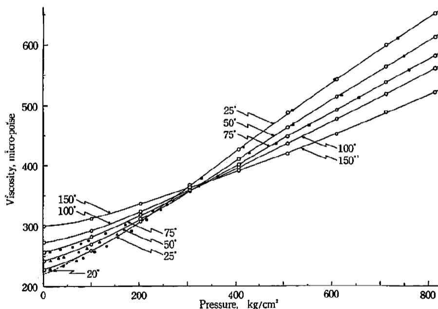
Fig. 1 Viscosity isotherms of argon
