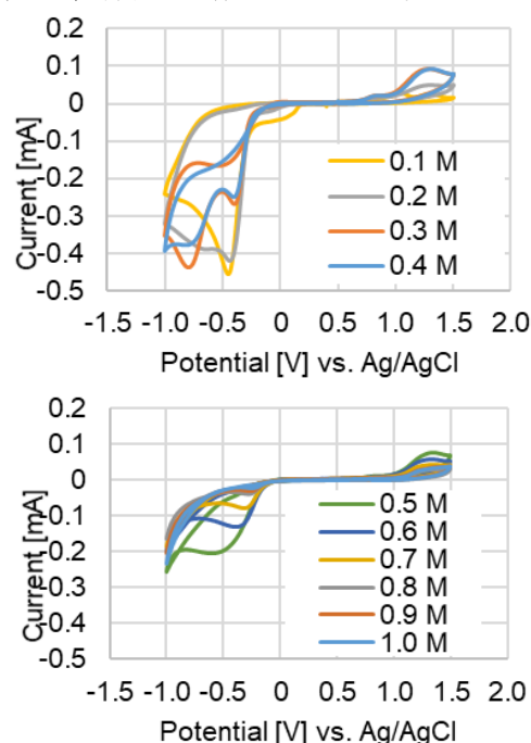
図 1 硝酸溶液中のモリブデンの CV 図の硝酸濃度依存性 ([Mo] = 10 mM, [HNO 3 ] = 0.1 ~ 1.0 M, Scanrate : 50 mV/s, )
