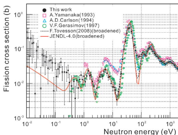
Fig.3 Neutron induced fission cross section of ^{237}\text{Np} using a lead spectrometer in LINAC facility.
