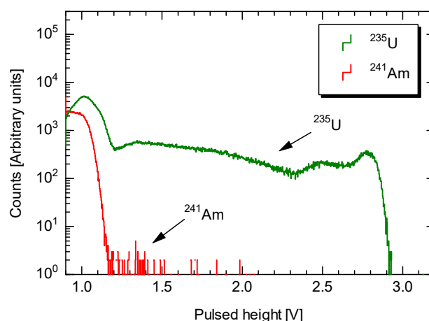
Fig. 4. Measured pulsed heights [4] of ^{241}\text{Am} and ^{235}\text{U} fission reaction rates at subcritical state.
