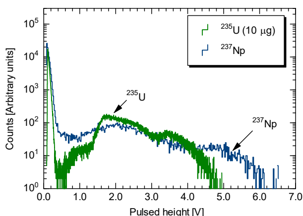
Fig. 3. Measured pulsed heights of ^{237}\text{Np} and ^{235}\text{U} fission reaction rates [3] in HEU-Pb zone (15, O; Fig. 1) at critical state.
