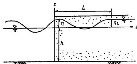
Fig. 3 Definition of groundwater level \eta with landward boundary conditions.
