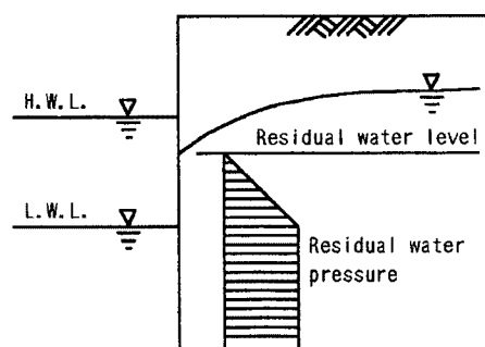
Fig. 4 Definition of residual water level around revetment.
