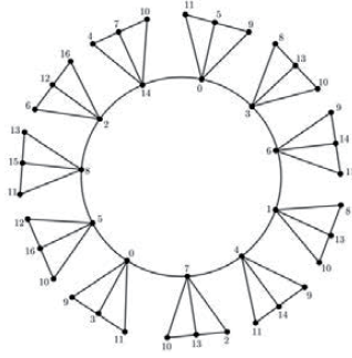
Figure 7: \lambda_{3,2,1}(C_{11} \odot P_3) = 16
