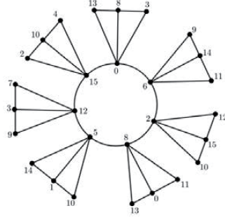
Figure 5: \lambda_{3,2,1}(C_7 \odot P_3) = 15
