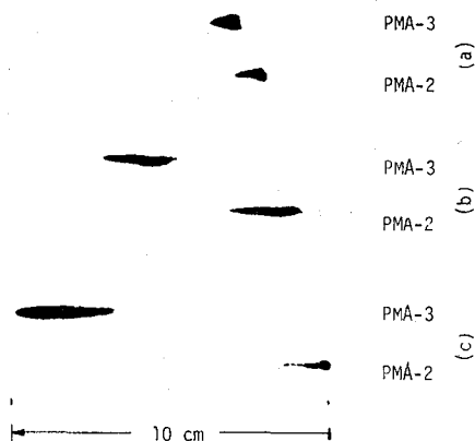
Fig. 3. Chromatographic behavior of PMA-2 and PMA-3 shown by equiellutropic binary developers, (a), (b), and (c). For the abbreviations, see text.
